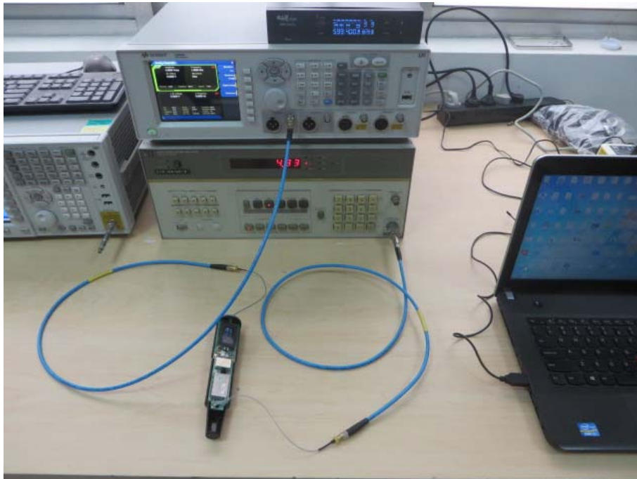
Conducted Test 2
