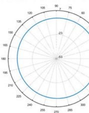
Total-3D-H-930MHZ
