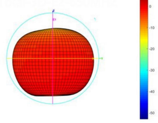
Total-3D-E2-920MHZ
