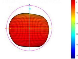
Total-3D-E1-920MHZ
