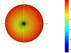
Total-3D-H-920MHZ
