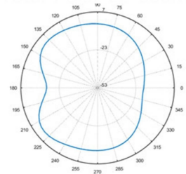
Total-Polar-E2-902MHZ
