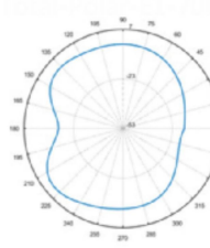
Total-Polar-E1-930MHZ
