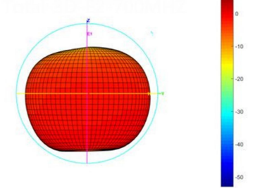
Total-3D-E2-930MHZ
