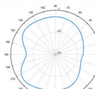
Total-Polar-E1-920MHZ
