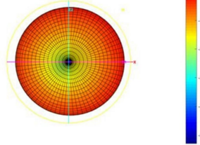
Total-3D-H-930MHZ
