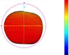
Total-3D-E1-930MHZ
