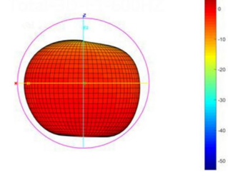
Total-3D-E1-902MHZ
