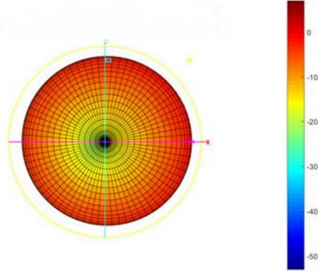
Total-3D-H-900MHZ
