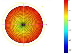
Total-3D-H-930MHZ
