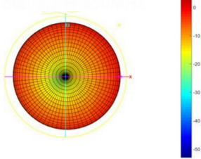
Total-3D-H-920MHZ
