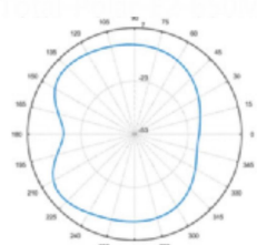
Total-Polar-E2-920MHZ
