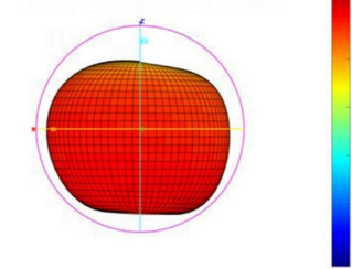
Total-3D-E1-920MHZ
