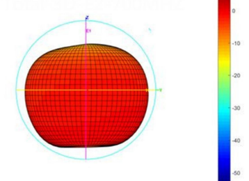
Total-3D-E2-930MHZ
