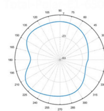
Total-Polar-E1-920MHZ
