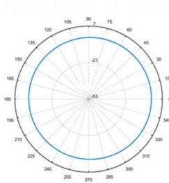
Total-Polar-H-902MHZ
