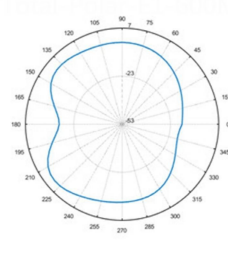
Total-Polar-E1-902MHZ
