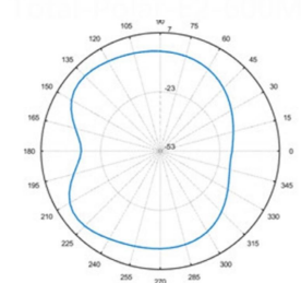
Total-Polar-E2-902MHZ
