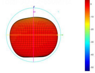
Total-3D-E2-920MHZ
