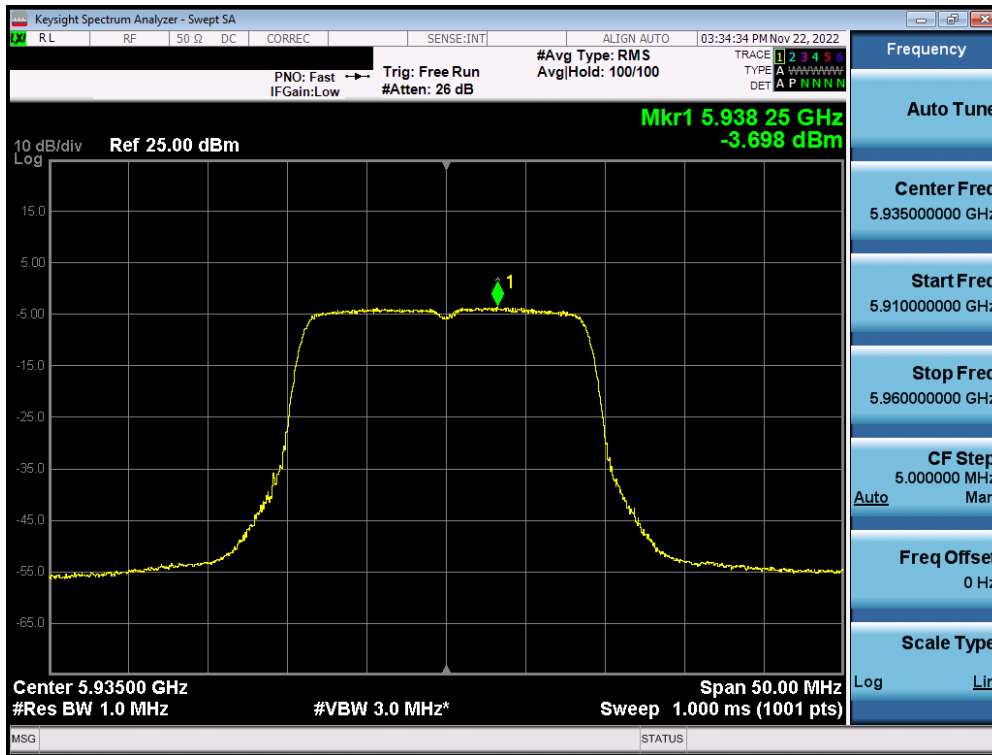
Plot 7-157. Power Spectral Density Measurement MIMO ANT2 (20MHz 802.11a (UNII Band 5) – Ch. 2)
