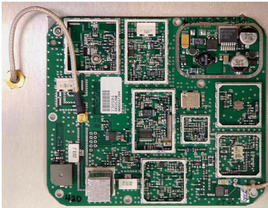
TRI2525B – PCB back view
