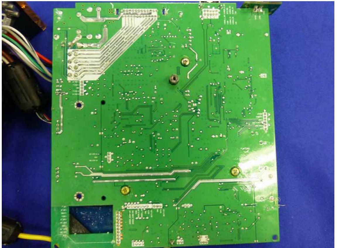
Figure 16 General Inside of the EUT
