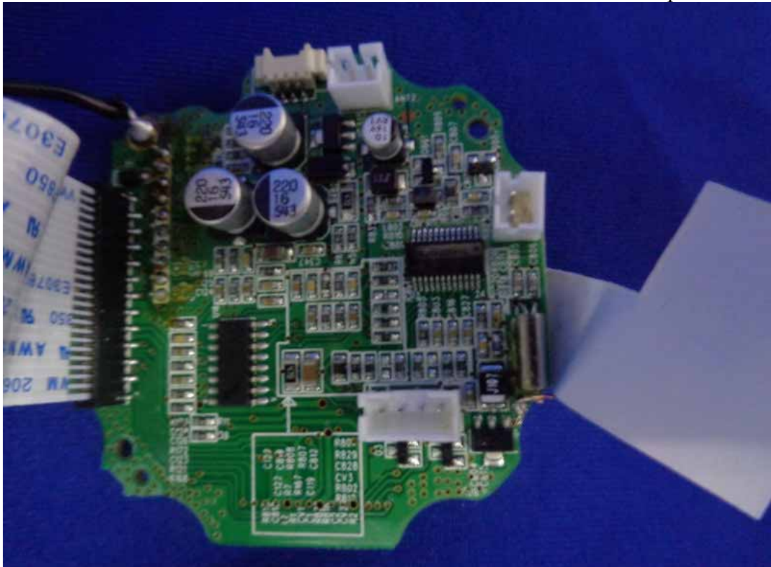
Figure 10 Component side of the PCB
