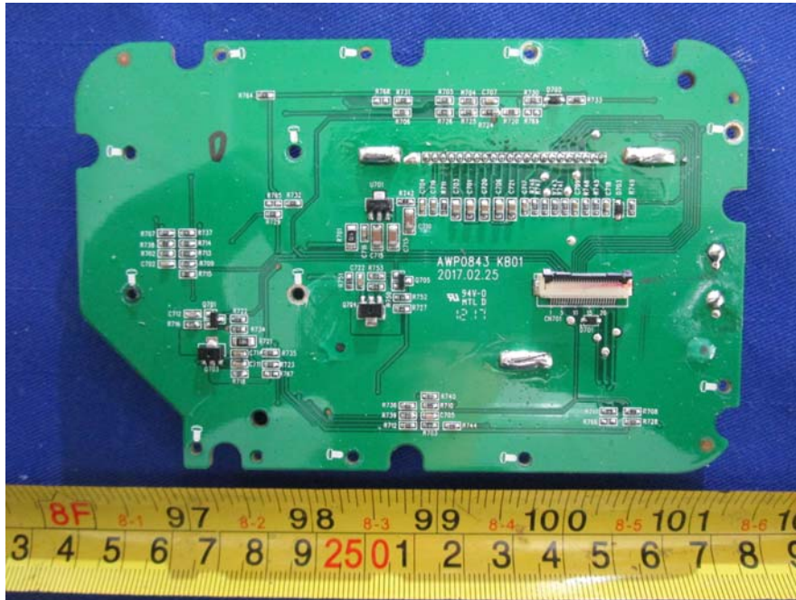
EUT –PCB Keyboard 01 Bottom View
