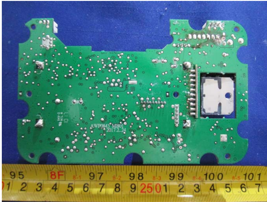
EUT – PCB Mainboard 01 Bottom View
