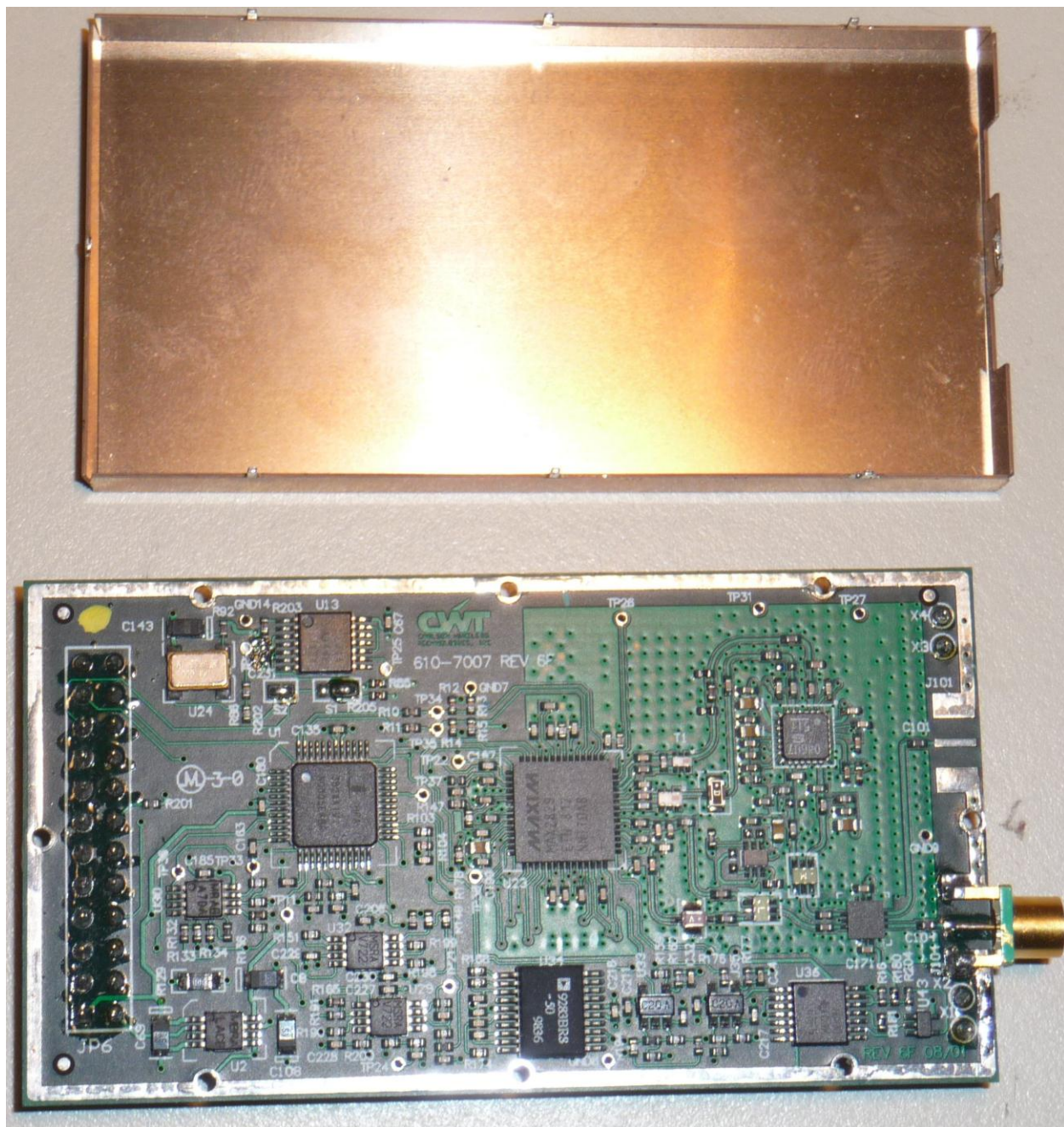
Photograph 14. Shield Radio
