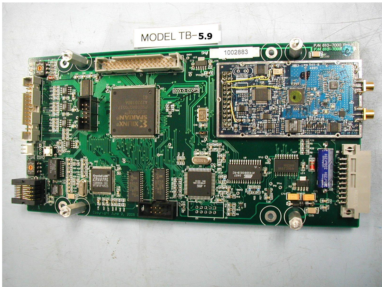
Photograph 13. Cover Off 5.9
