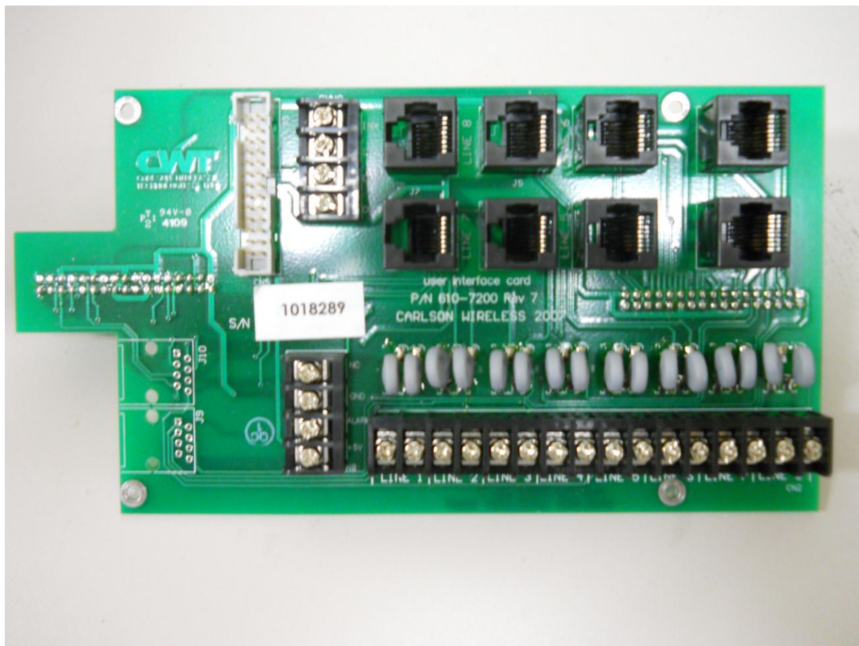
Photograph 8. Card 1 Front
