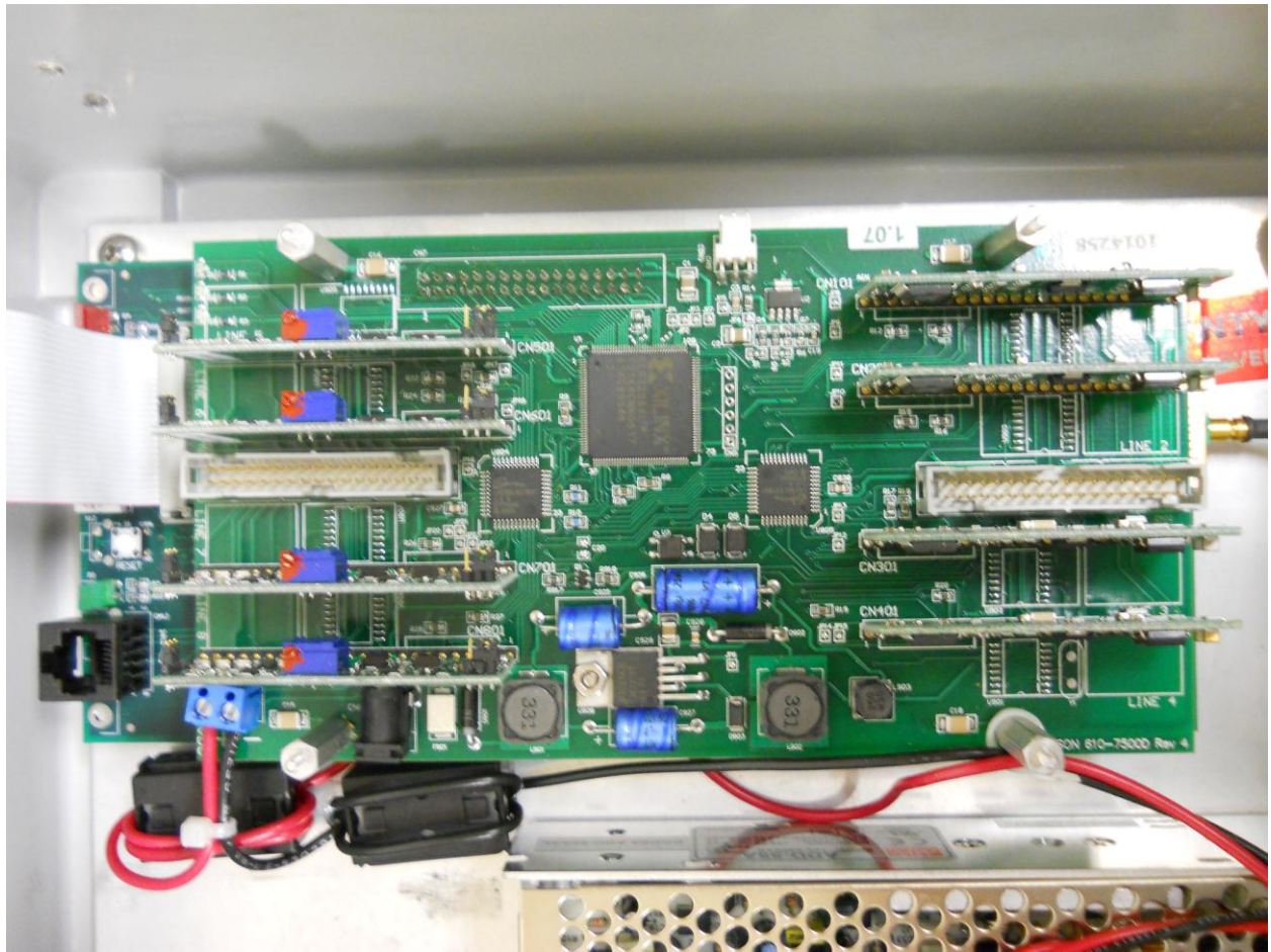
Photograph 3. Layer 2
