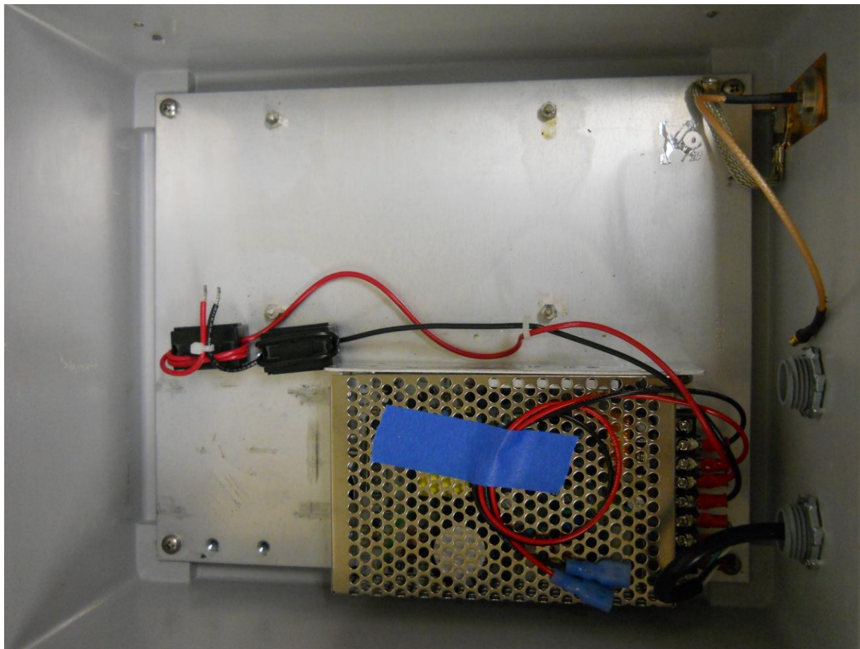
Photograph 6. PSU
