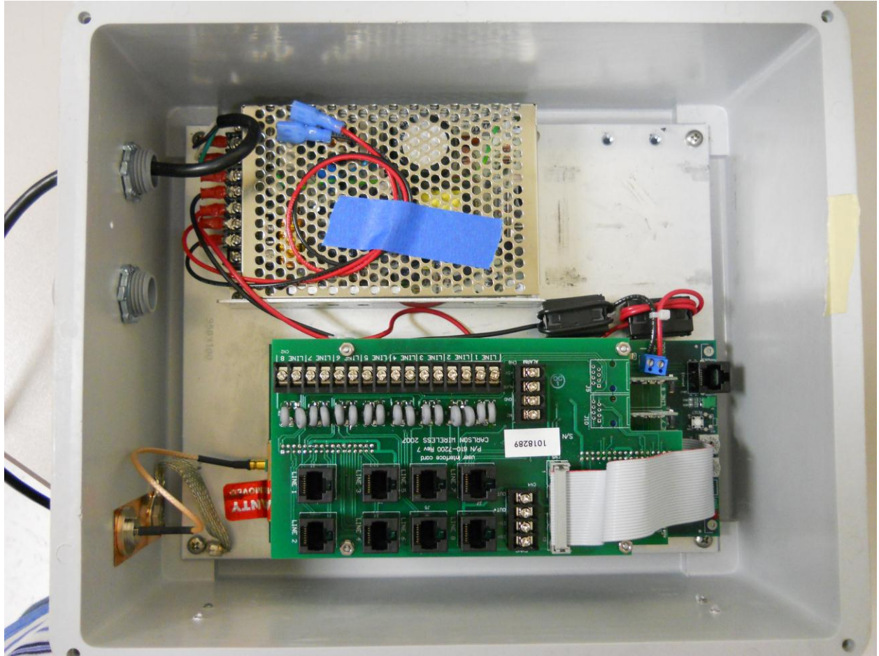
Photograph 5. Opened (Layer 1)
