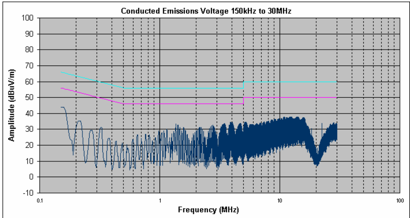
Conducted Emission, Phase Line Plots– TB 2.4-5.8 (5750-5825 MHz)
