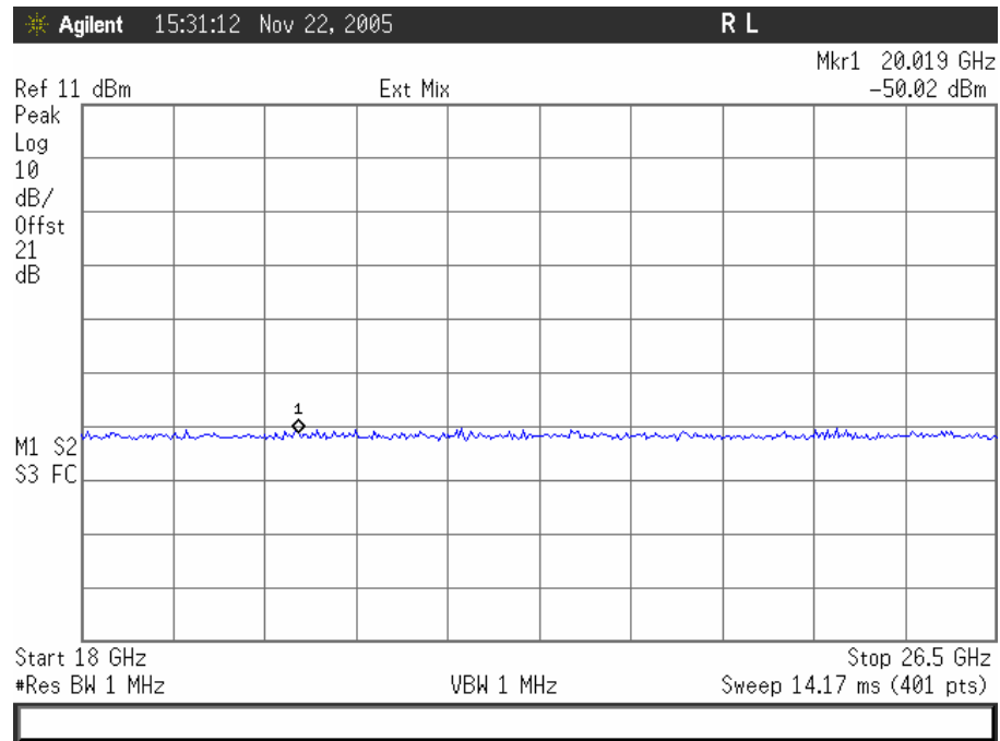
Plot 18. 802.11/a – Low Channel Conducted Emissions 18 -26.5GHz
