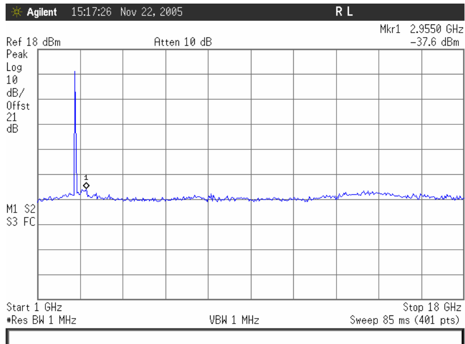
Plot 14. 802.11/g – High Channel Conducted Emissions 1-18GHz
