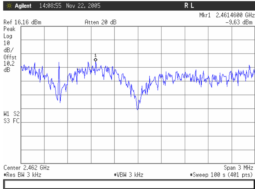
Plot 34. 802.11/g – High Ch Peak Power Spectral Density
