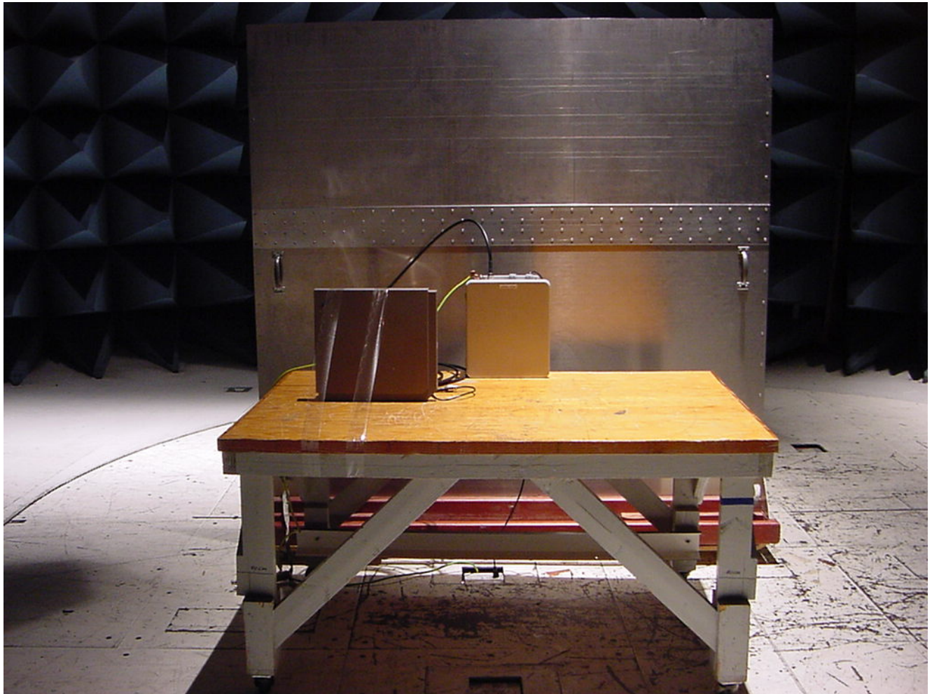
Photograph 5. Conducted Emissions TB 2.4-5.8 (2400-2483.5 MHz) Test Setup
