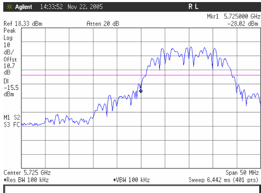
Plot 30. 802.11/a – Lower Band Edge
