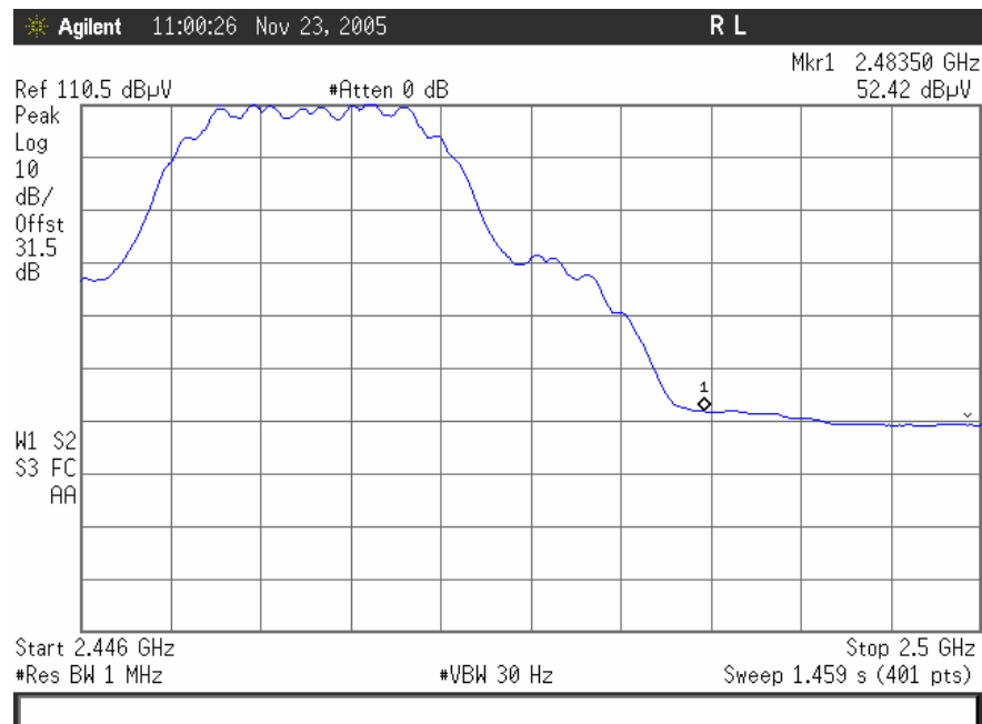
Plot 6. 802.11/g radiated restricted band 2483.5 – 2500MHz Peak
