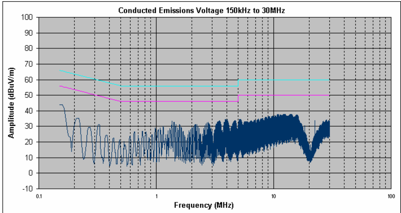
Conducted Emission, Phase Line Plots– TB 2.4-5.8 (2400-2483.5 MHz)
