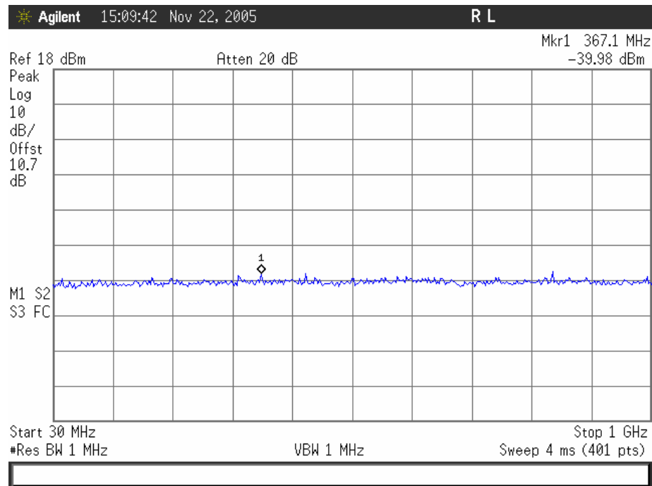
Plot 13. 802.11/g – High Channel Conducted Emissions 30MHz – 1GHz
