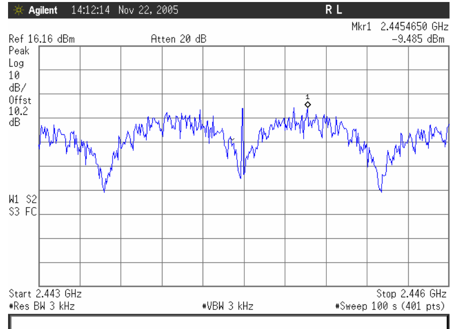
Plot 33. 802.11/g – Mid Ch Peak Power Spectral Density
