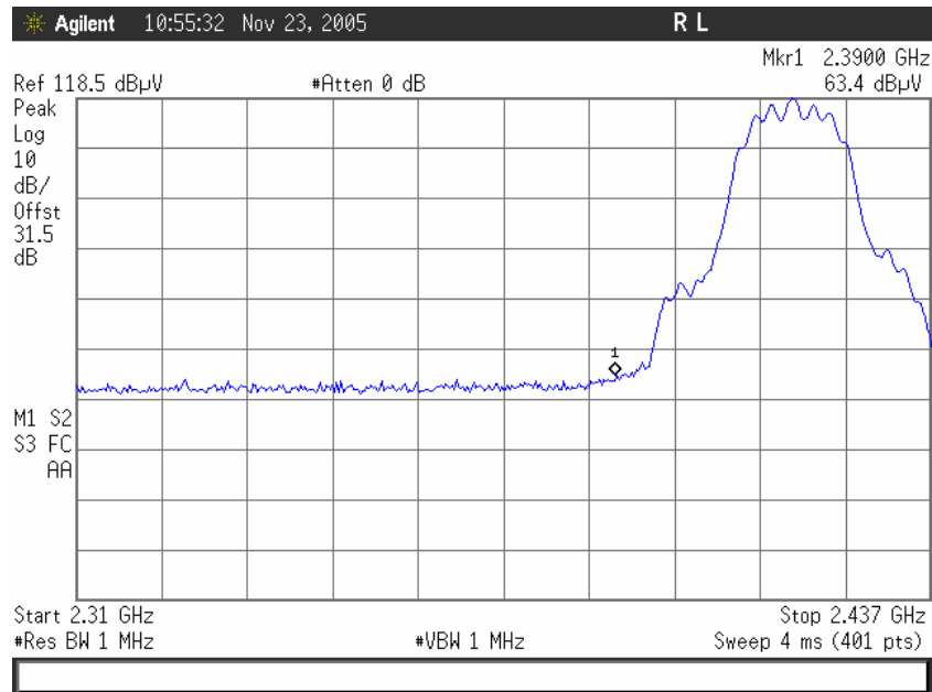
Plot 3. 802.11/g radiated restricted band 2310- 2390 MHz Peak
