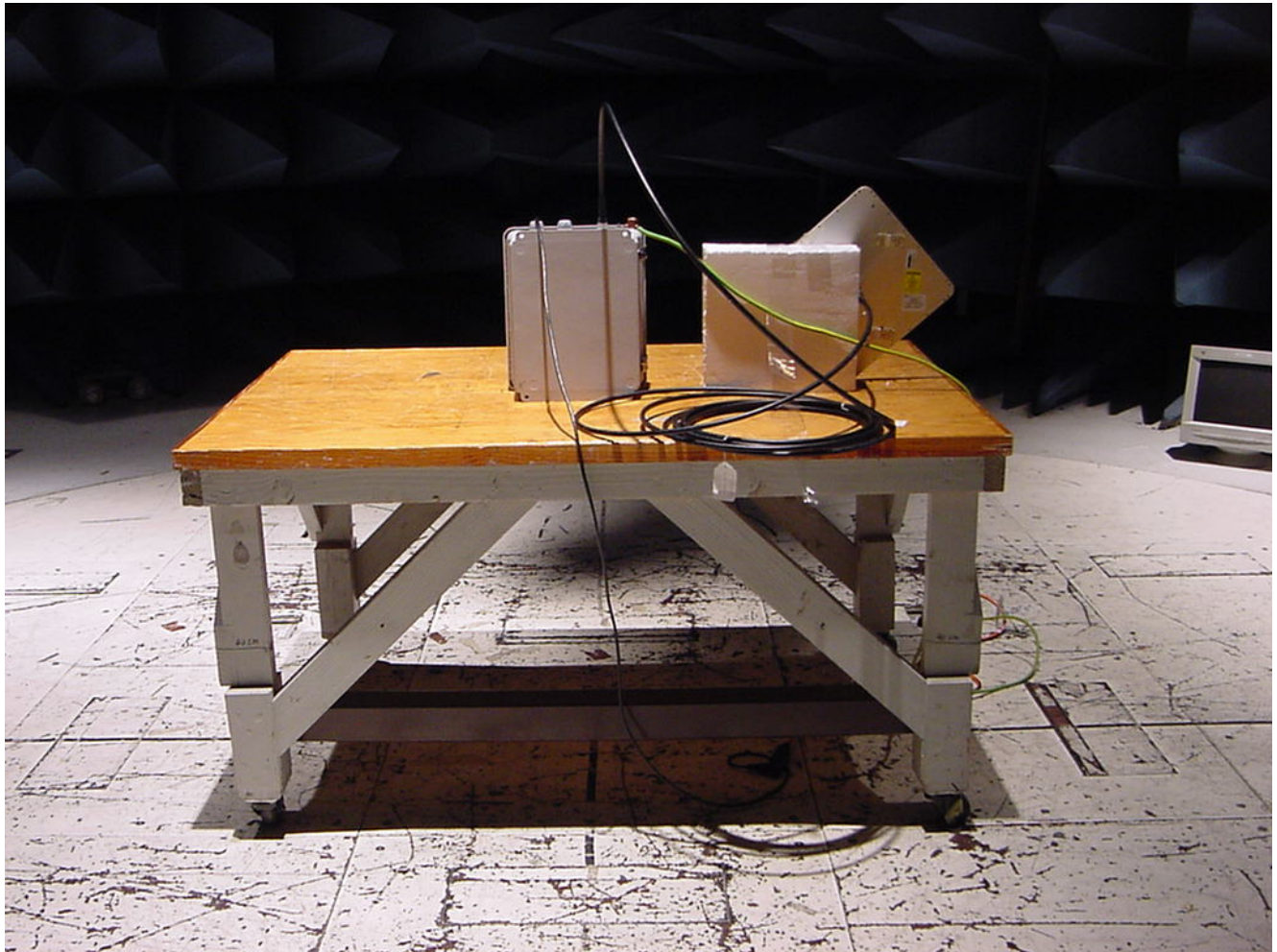
Photograph 4. Radiated Emission TB 2.4-5.8 (5750-5825 MHz) Test Setup
