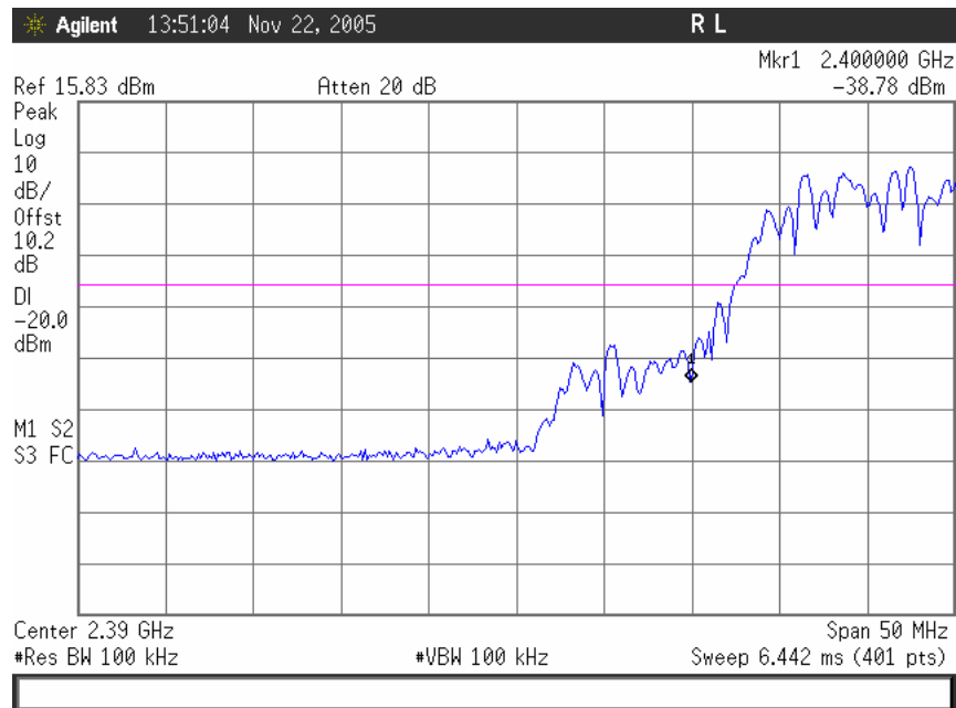
Plot 28. 802.11/g – Lower Band Edge
