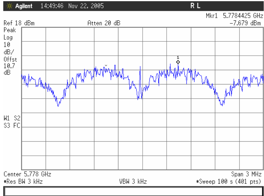
Plot 36. 802.11/a – Mid Ch Peak Power Spectral Density
