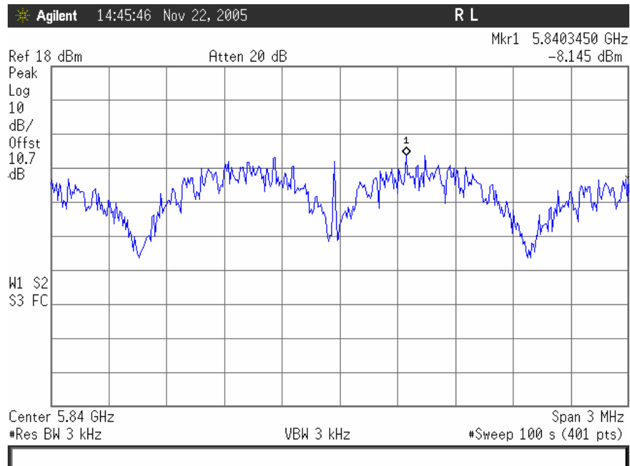
Plot 37. 802.11/a – High Ch Peak Power Spectral Density
