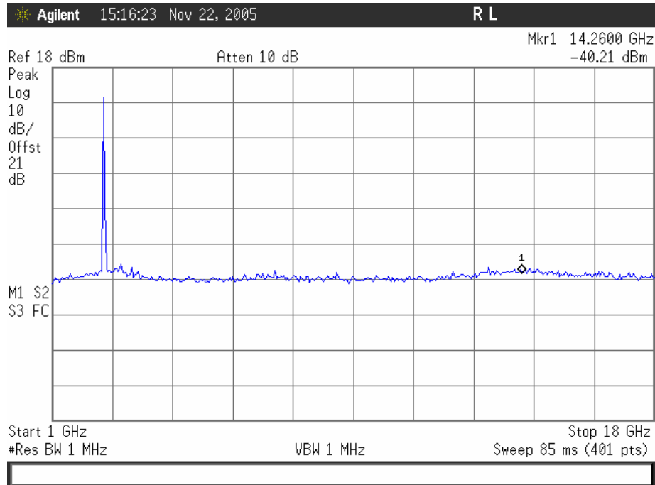
Plot 11. 802.11/g – Mid Channel Conducted Emissions 1-18GHz
