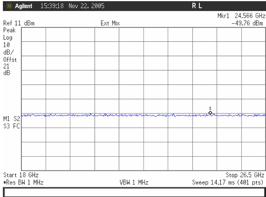
Plot 9. 802.11/g – Low Channel Conducted Emissions 18 – 26.5GHz
