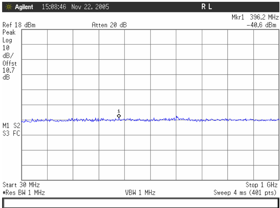
Plot 10. 802.11/g – Mid Channel Conducted Emissions 30MHz – 1GHz
