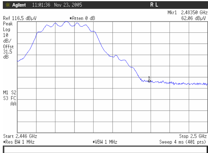
Plot 5. 802.11/g radiated restricted band 2483.5 – 2500MHz Peak
