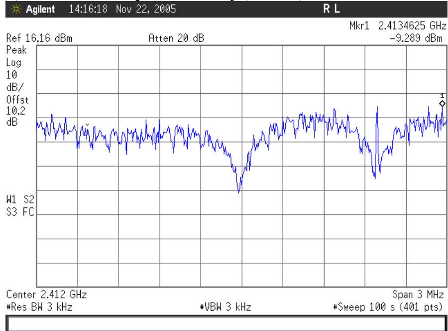
Plot 32. 802.11/g – Low Ch Peak Power Spectral Density
