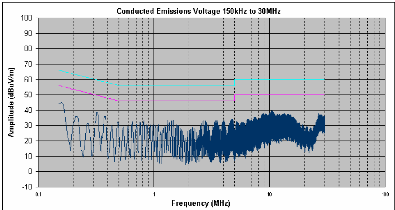
Conducted Emission, Neutral Line Plots– TB 2.4-5.8 (2400-2483.5 MHz)
