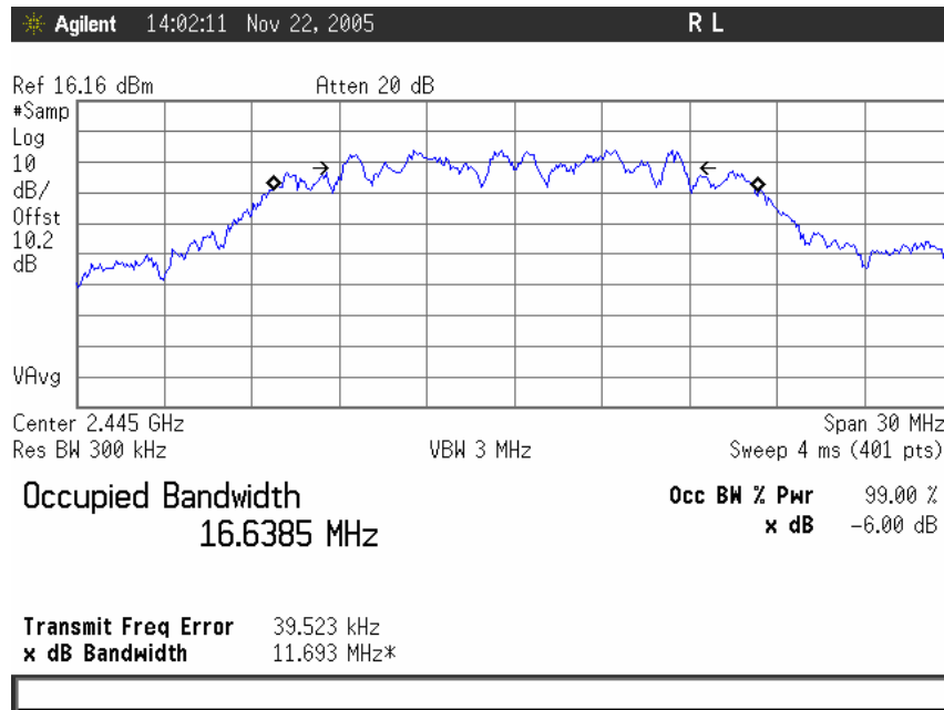
Plot 1. 802.11/g Mid Ch Occupied Band Width
