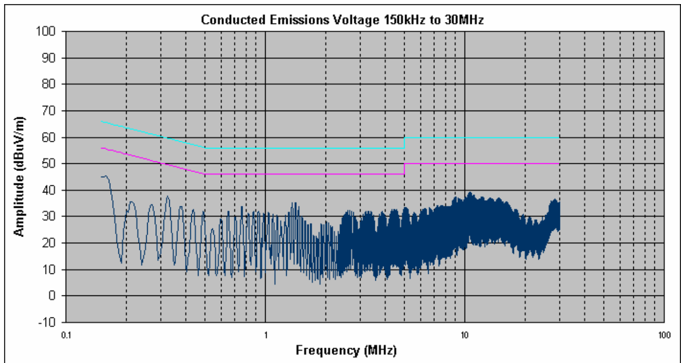
Conducted Emission, Neutral Line Plots– TB 2.4-5.8 (5750-5825 MHz)
