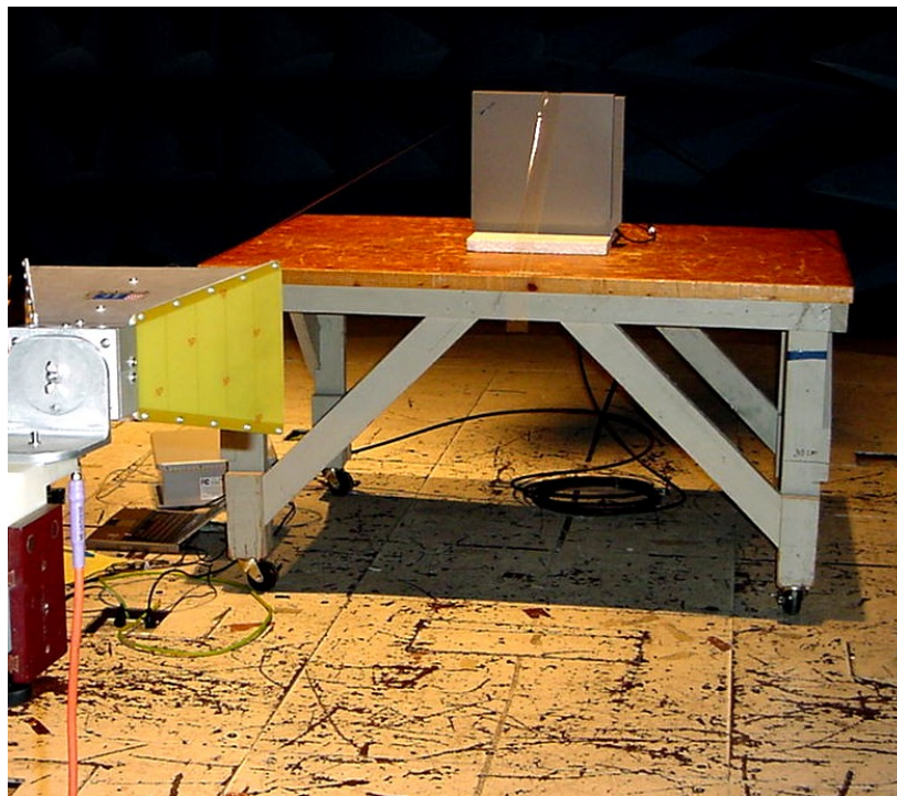
Photograph 3. Test Equipment and setup for various Radiated Measurements
