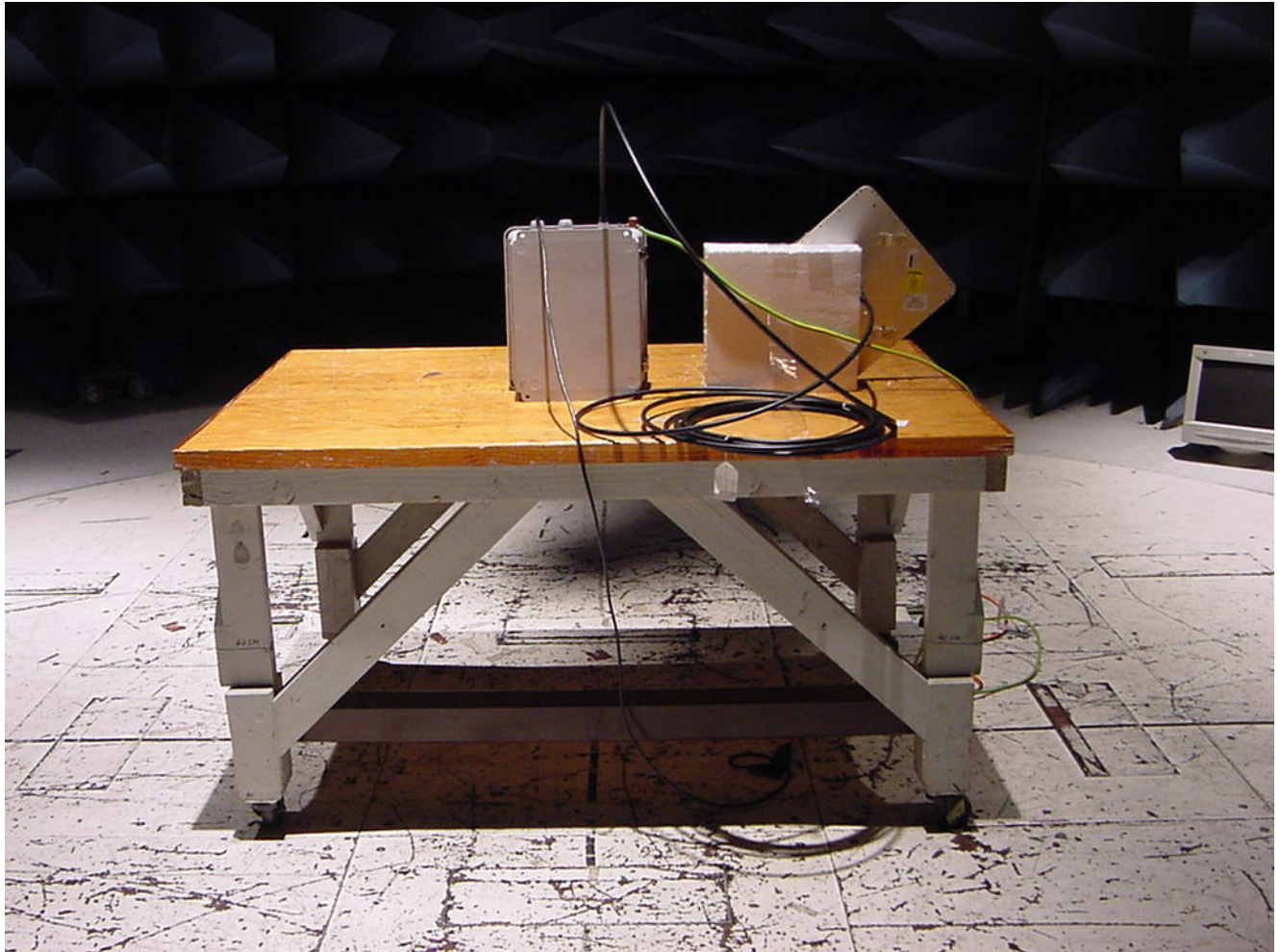
Photograph 8. Radiated Emission Limits TB 2.4-5.8 (5750-5825 MHz) Test Setup
