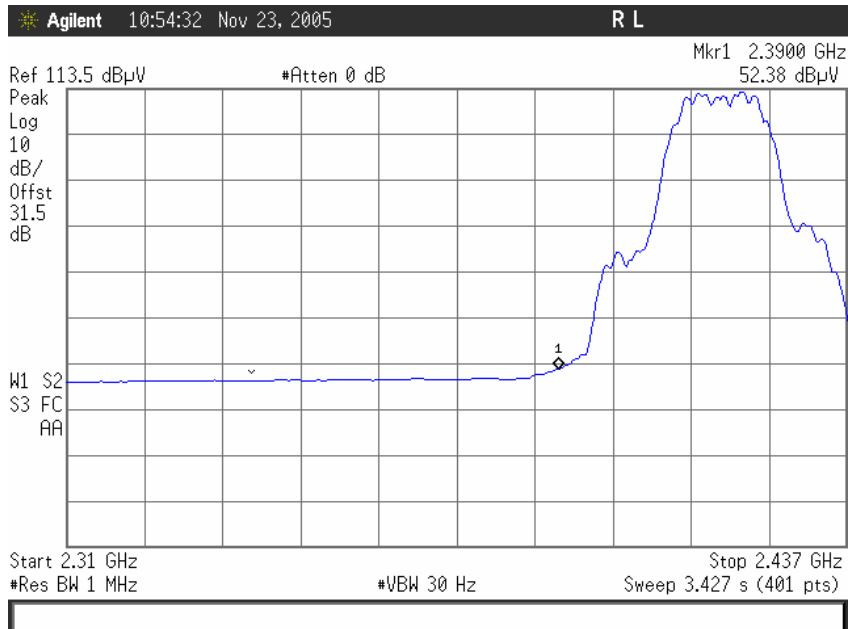
Plot 4. 802.11/g radiated restricted band 2310- 2390 MHz Avg
