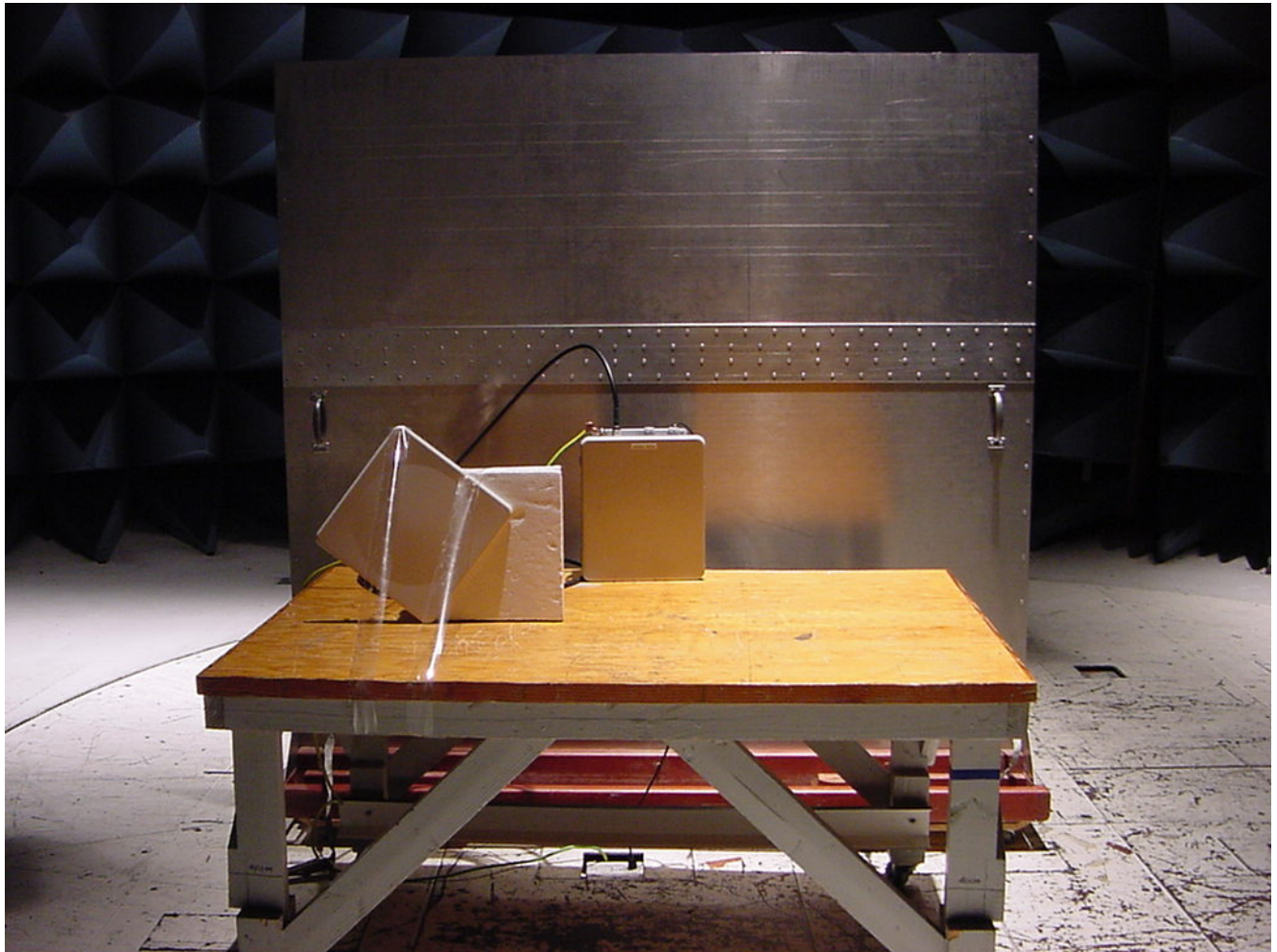
Photograph 6. Conducted Emissions TB 2.4-5.8 (5750-5825 MHz) Test Setup
