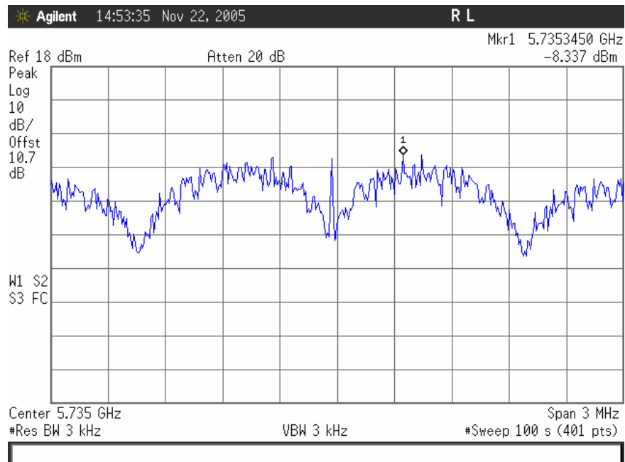
Plot 35. 802.11/a – Low Ch Peak Power Spectral Density
