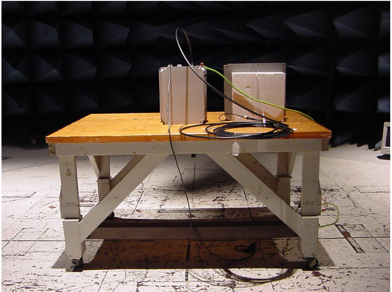
Photograph 3. Radiated Emission TB 2.4-5.8 (2400-2483.5 MHz) Test Setup
