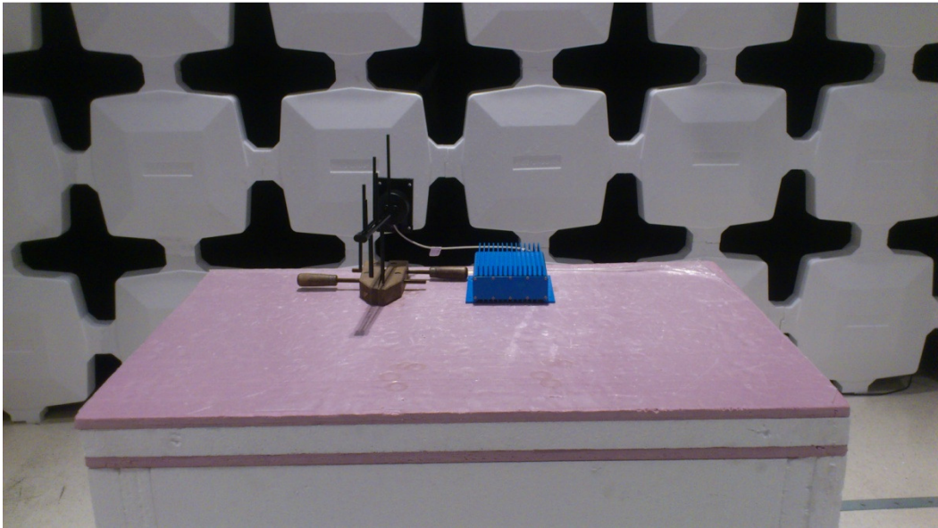
Radiated test setup photo #2
