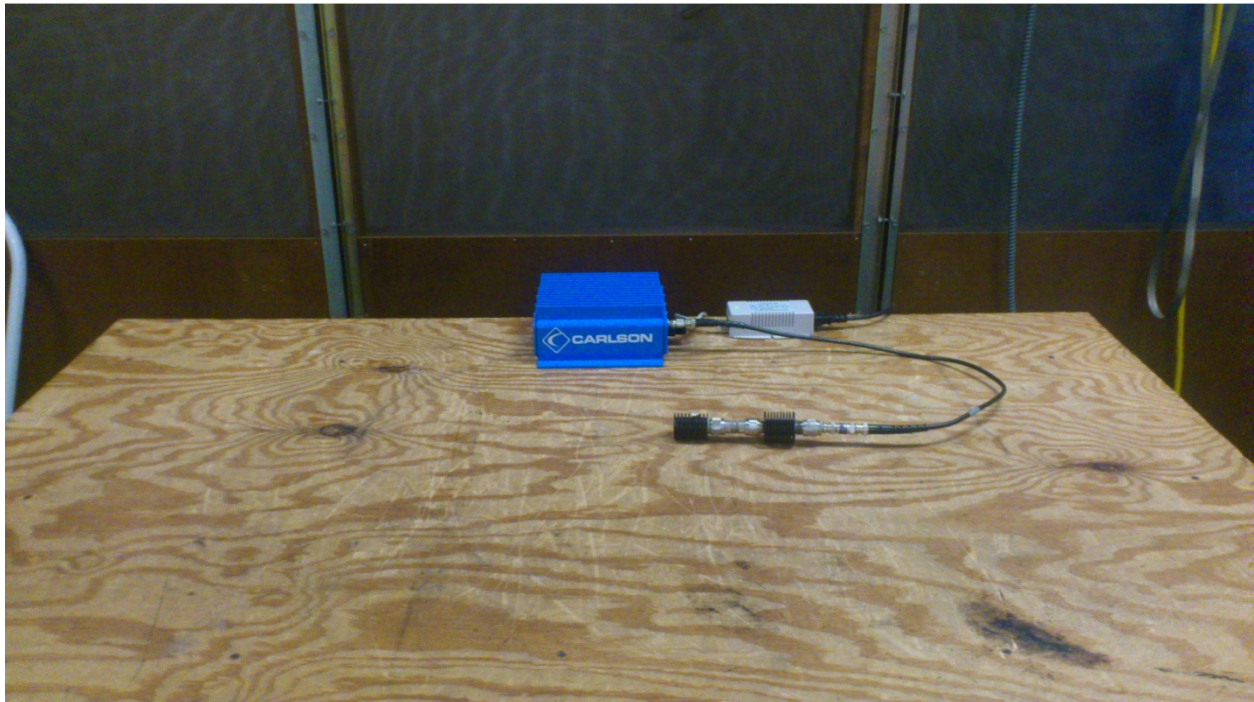
Powerline conducted test setup photo 1
