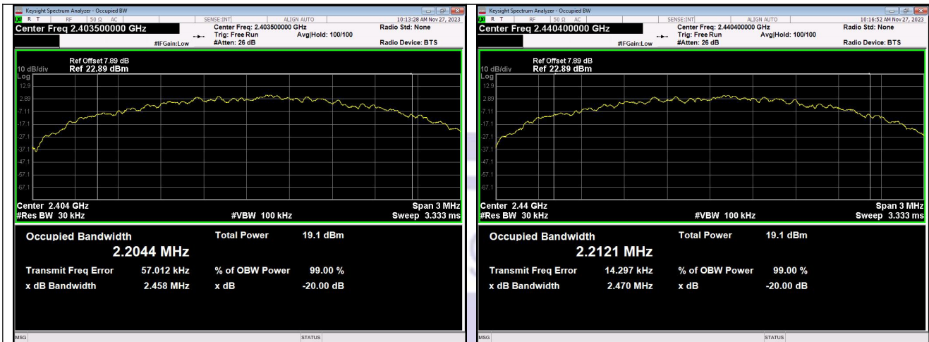
FSK_Channel 0
