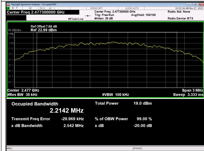
FSK_Channel 48
