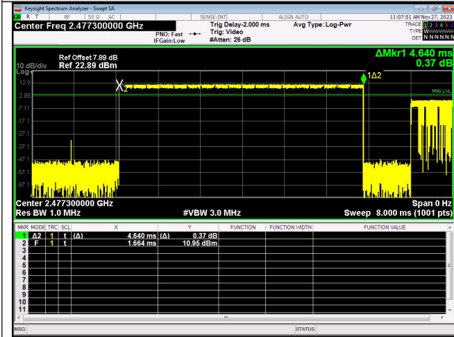
Pulse Width FSK
