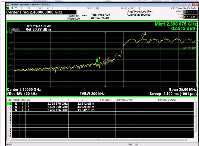
Out Of Band Emission FSK_Channel 48
