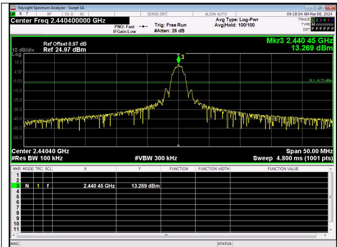
Out Of Band Emission FSK_Channel 24
