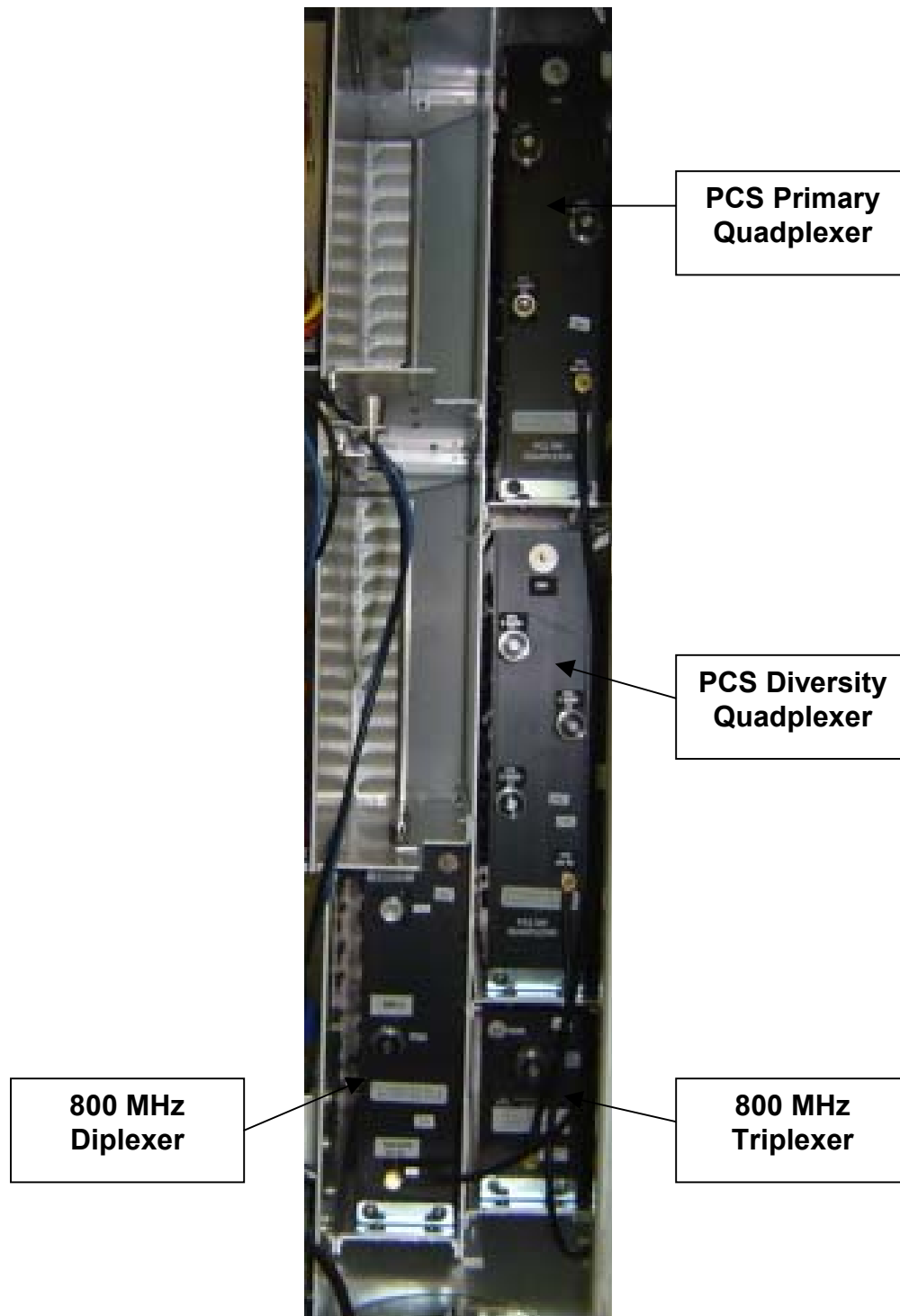
Figure 7-3 Multiplexers installed in RAN
