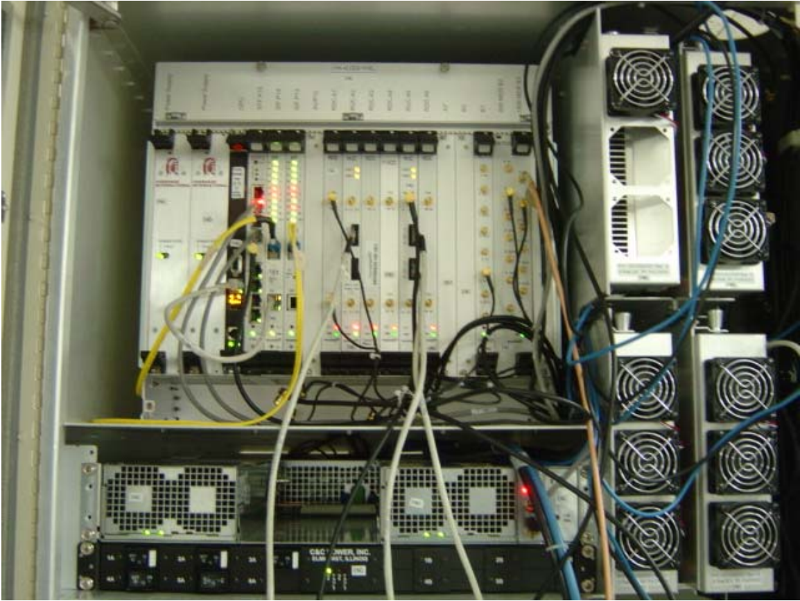
Figure 7-2 RAN Compact PCI chassis
