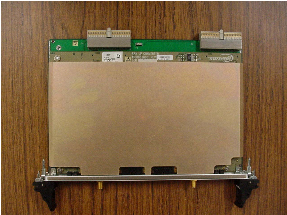
Figure 7-10 RUC Module, Top View
