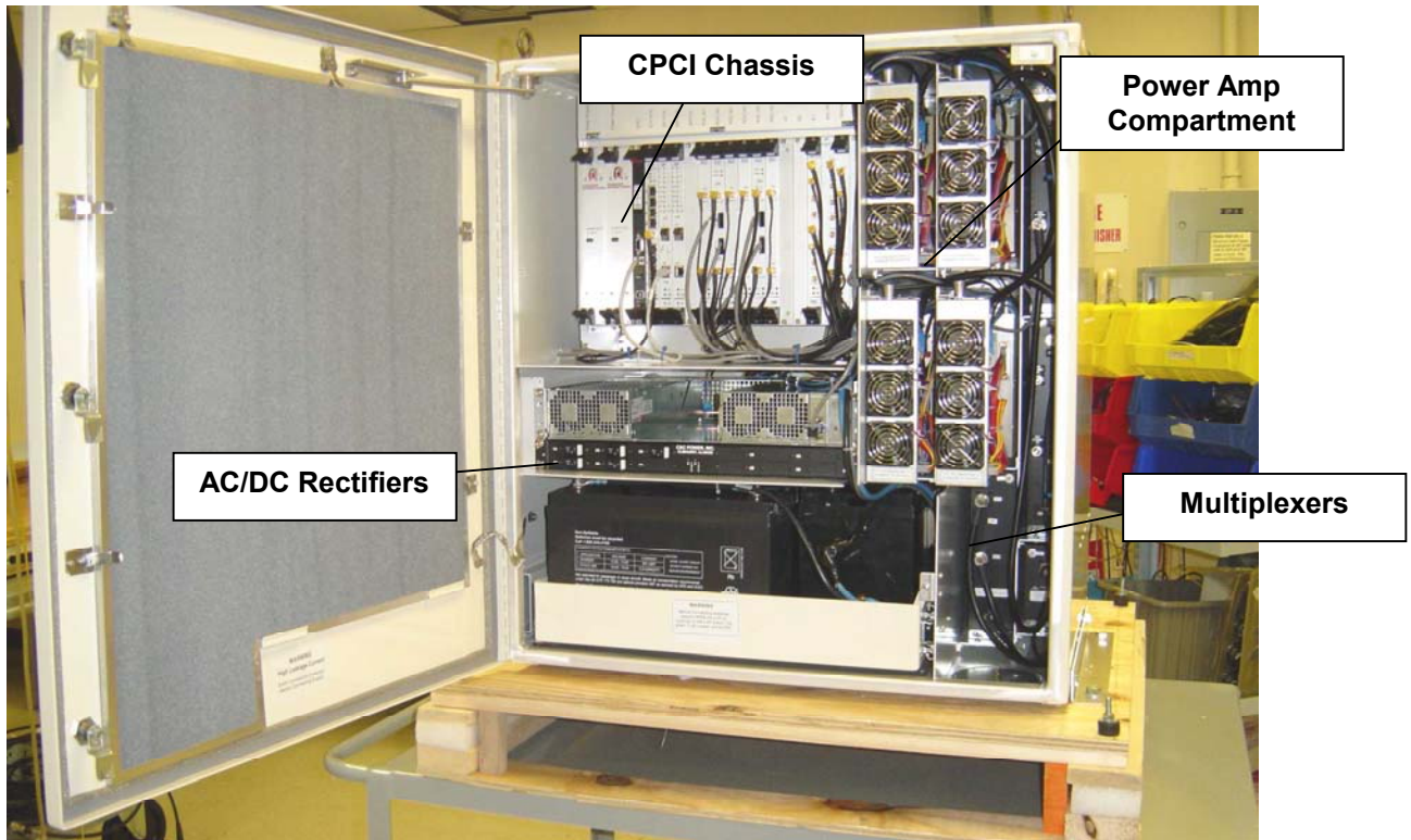
Figure 7-1 RAN, door open
