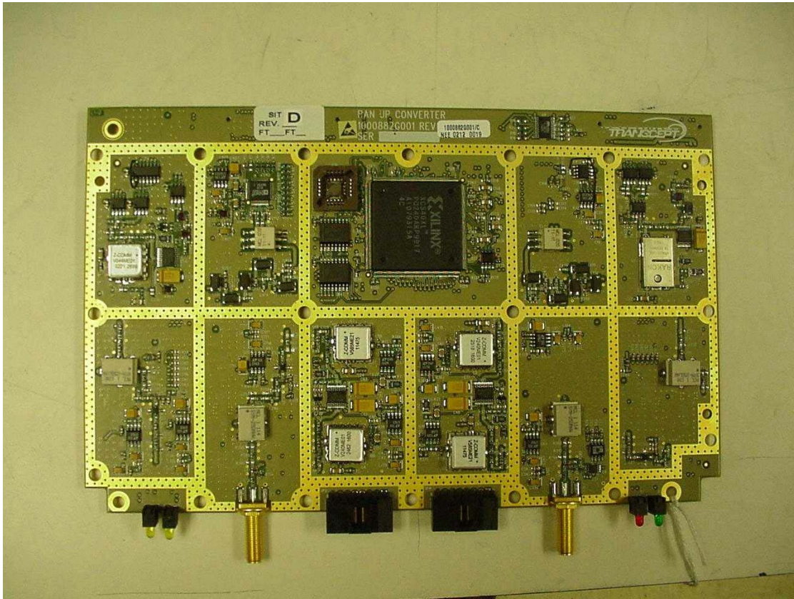
Figure 7-11 RUC circuit card (shield removed)
