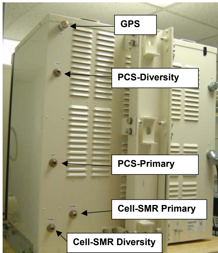
Figure 6-3 Detail of RF Connector Identification on Rear of RAN
