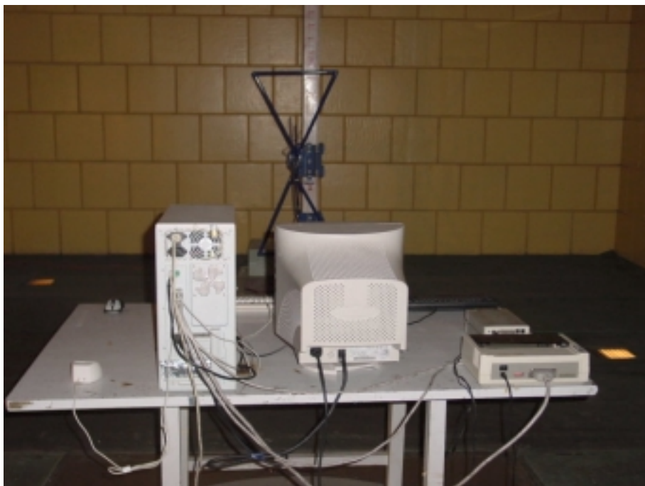
BACK VIEW OF RADIATED MEASUREMENT
