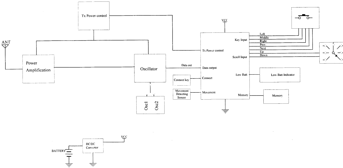
P2402 Mouse Block Diagram
