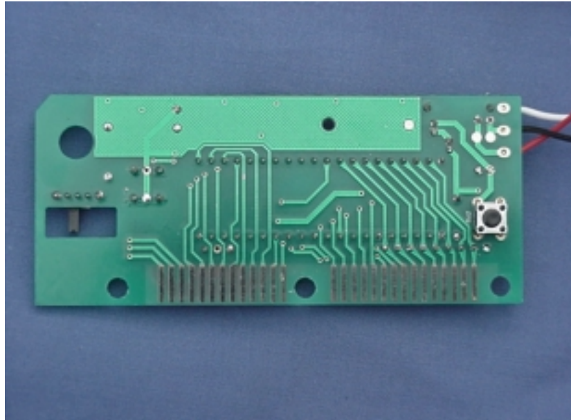
FIGURE 4 PCB of the EUT, (Rear View)
