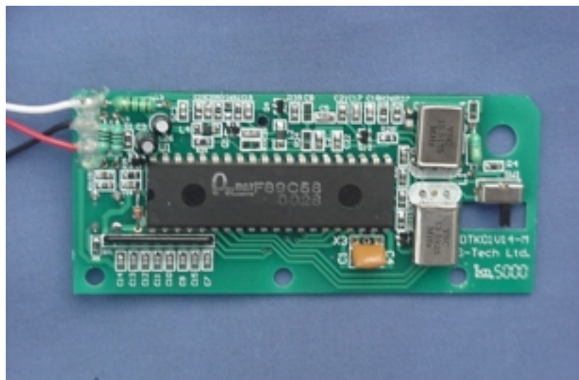
FIGURE 3 PCB of the EUT, (Front View)
