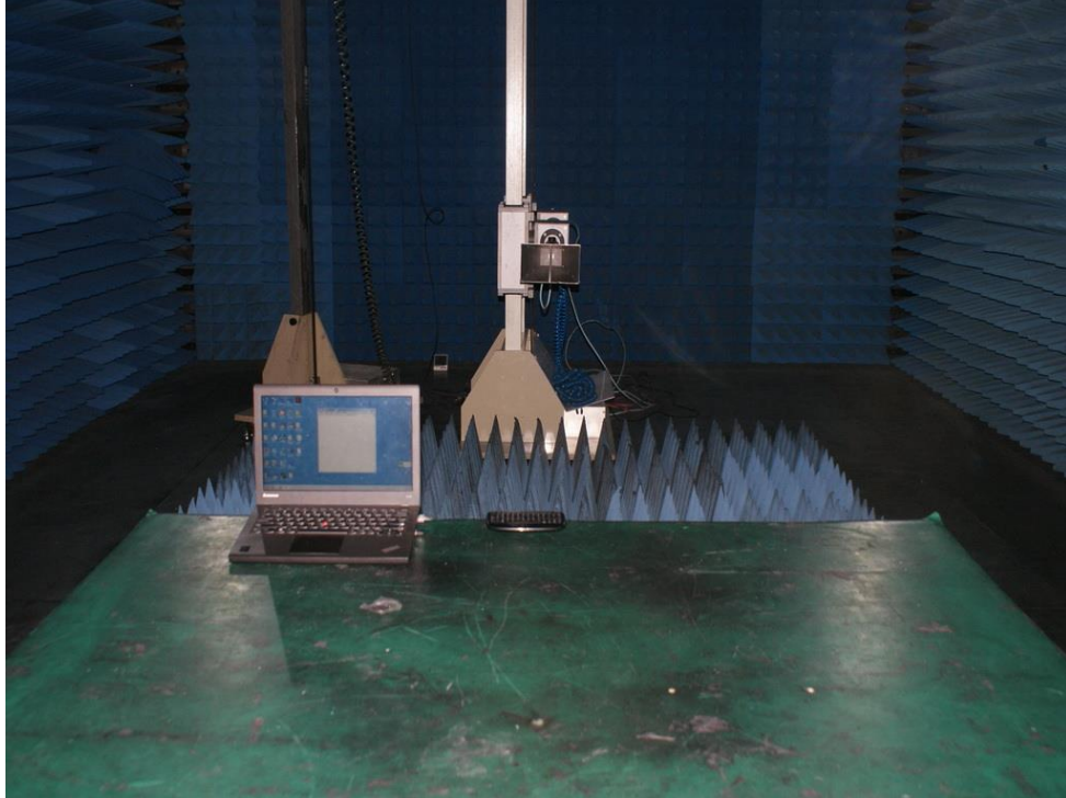
Photograph 7: Set-up for Radiated Emission (1GHz ~ 6GHz)
