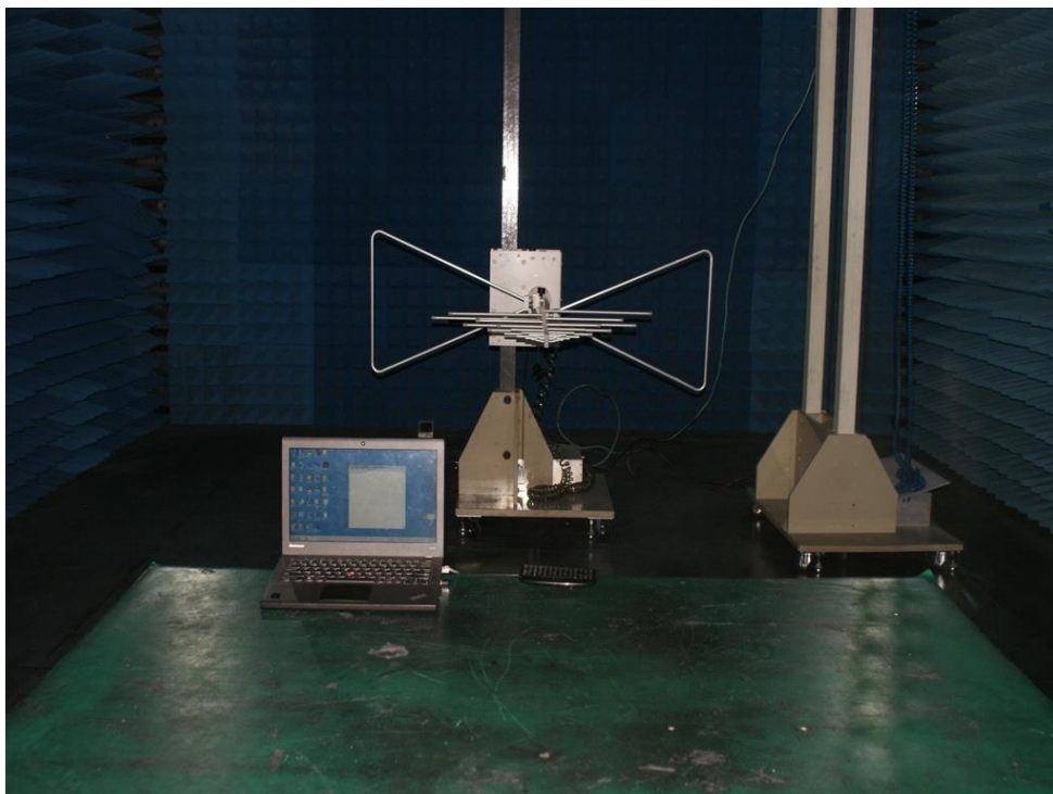
Photograph 6: Set-up for Radiated Emission (30MHz ~ 1GHz)
