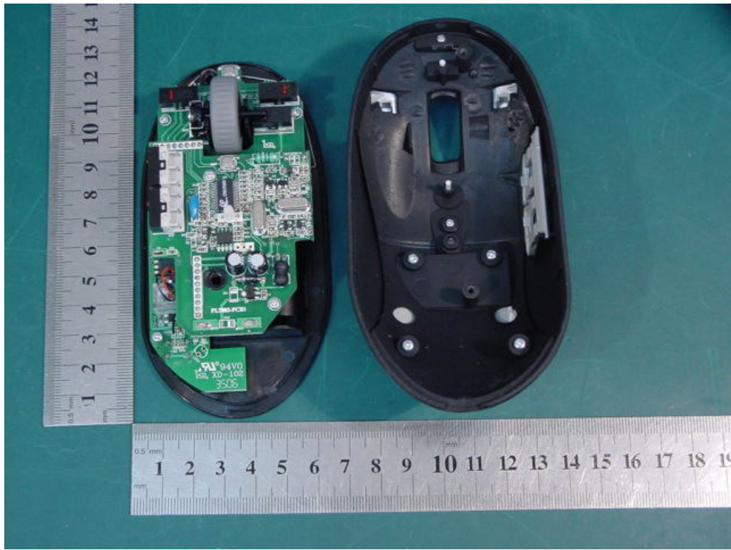
Wireless Mouse PL7802 internal photo
