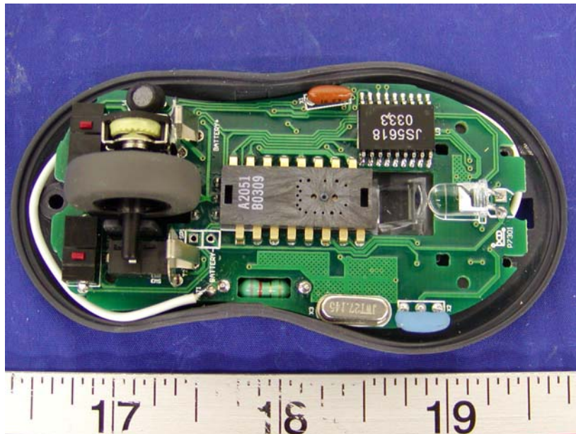
Transmitter – Component View
