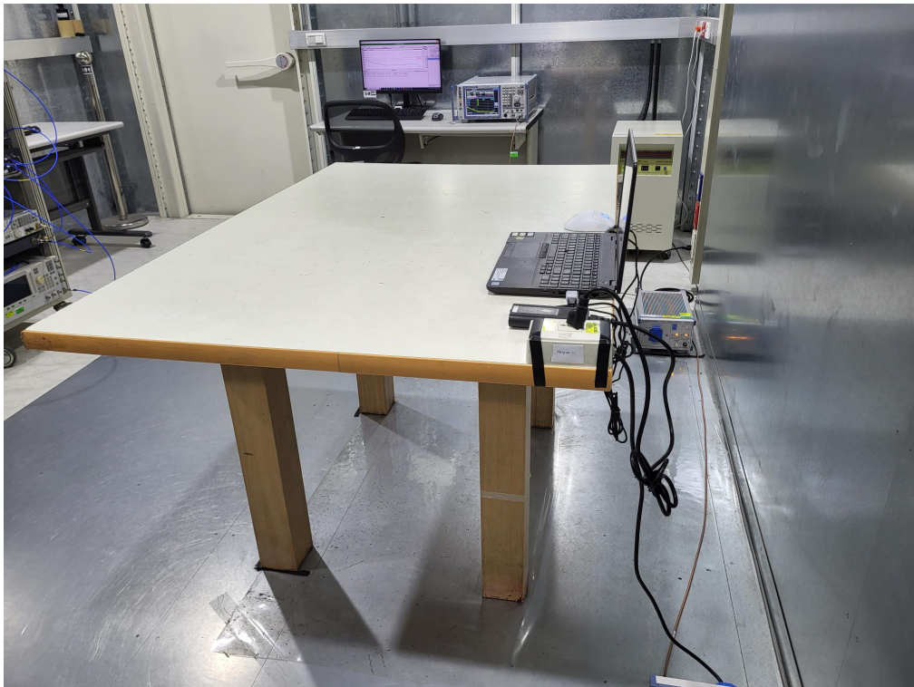
Back View of AC Power Line Conducted Emission
