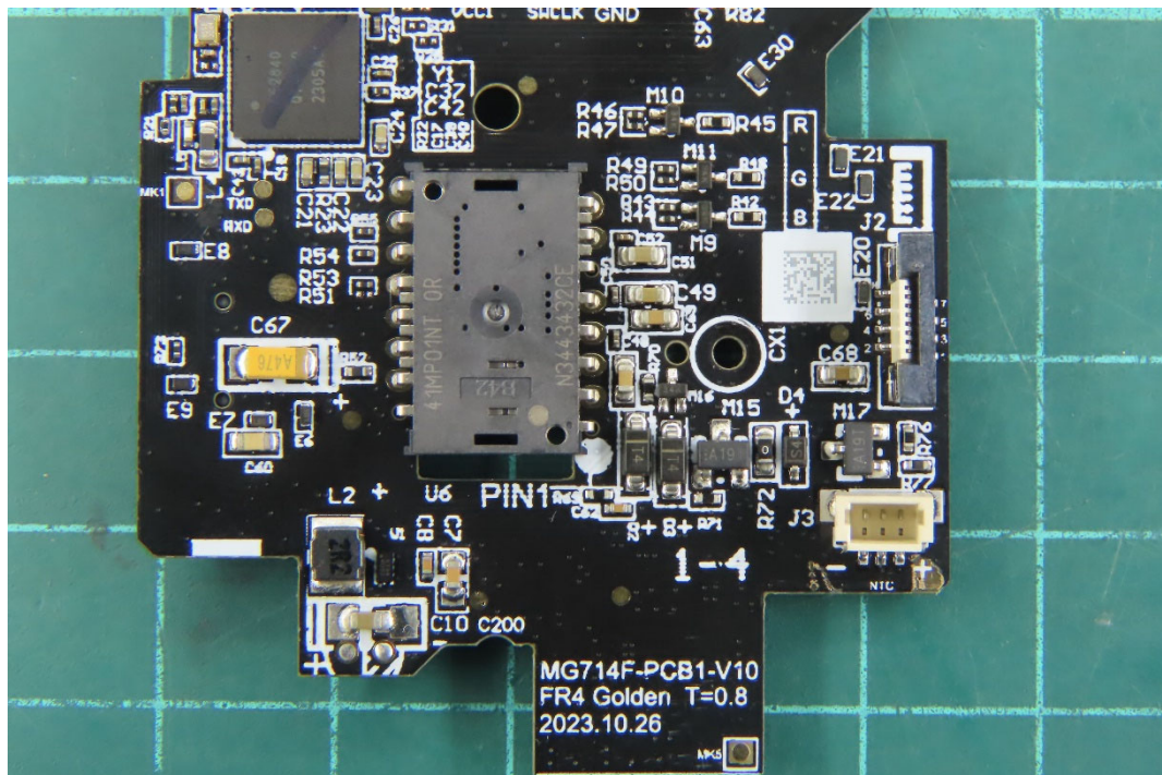
(29)EUT Photo
