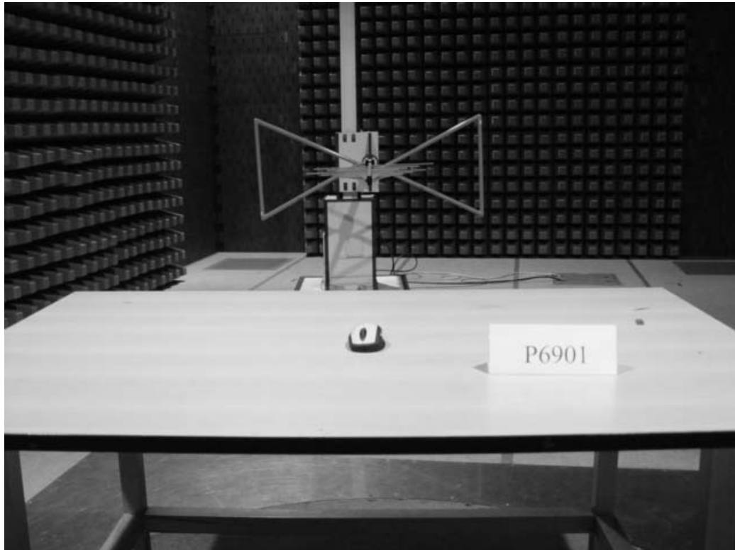
Photograph 3: Set-up for Radiation Measurement below 1GHz
