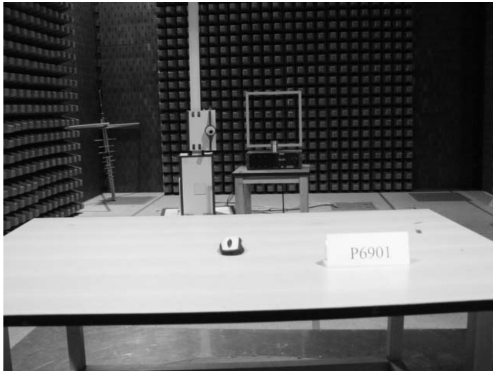
Photograph 2: Set-up for Radiation Measurement Below 30MHz
