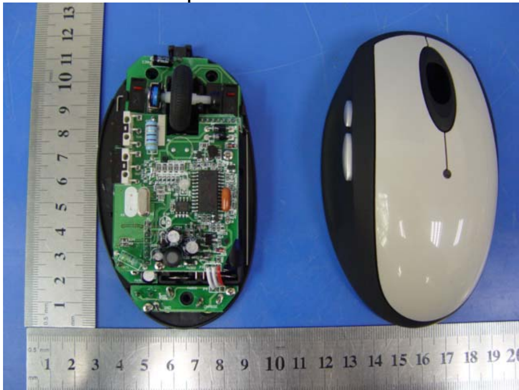
Wireless mouse P6901 internal photo
