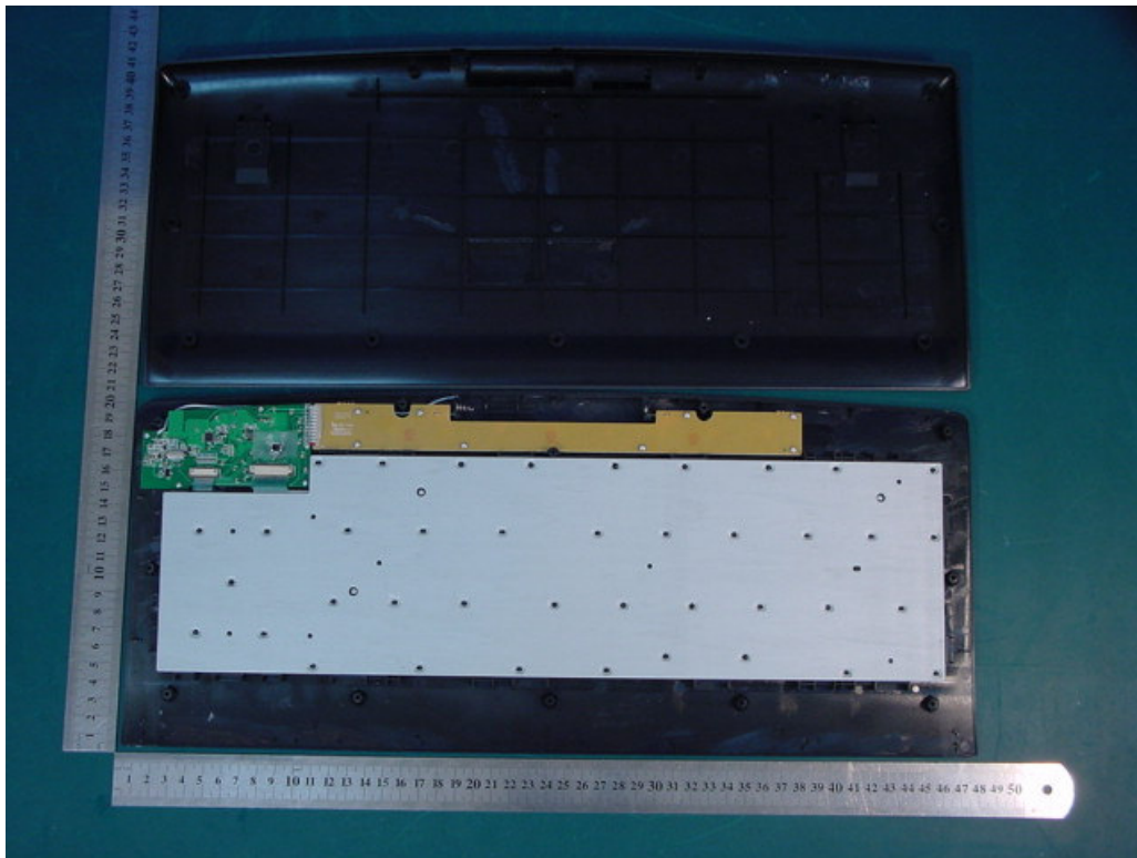
Wireless Keypad HT03 internal photo
