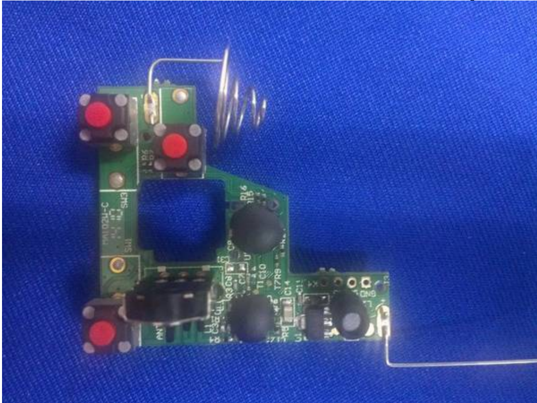
Figure 7 Component Side of the PCB
