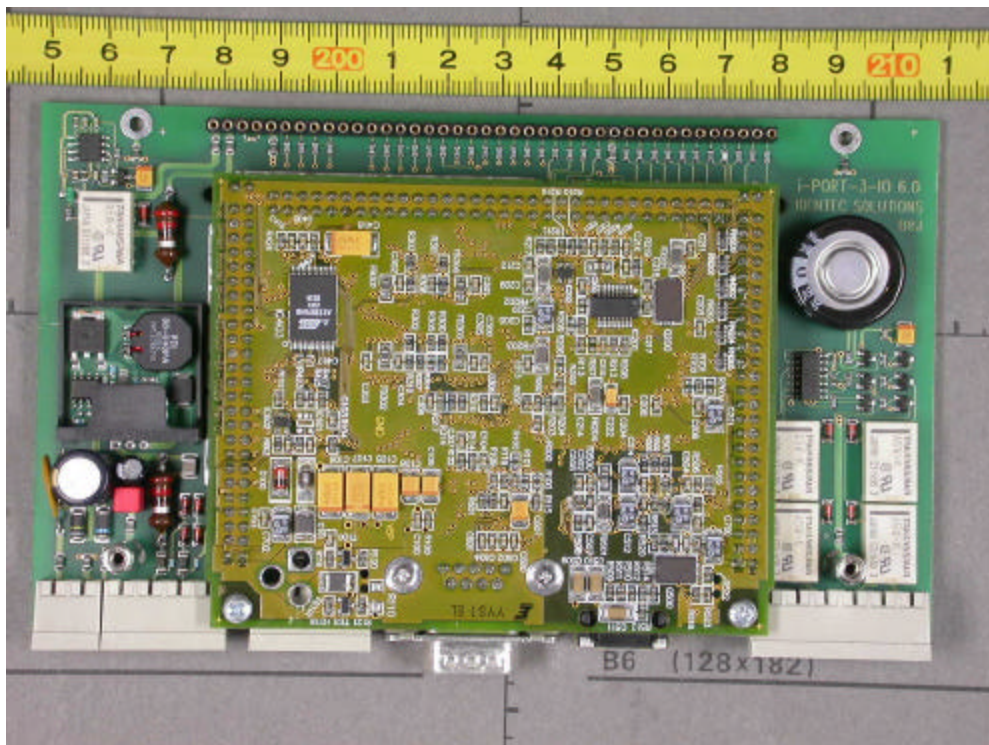
Top view - printed board ( Host section )
