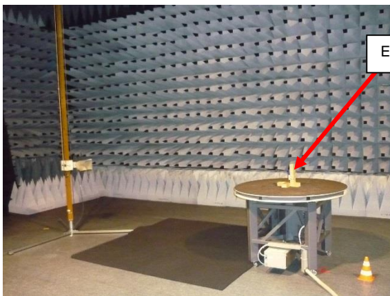
receiving/transmitting tested frequencies above 1 GHz (according to ANSI C63.10-2009)
