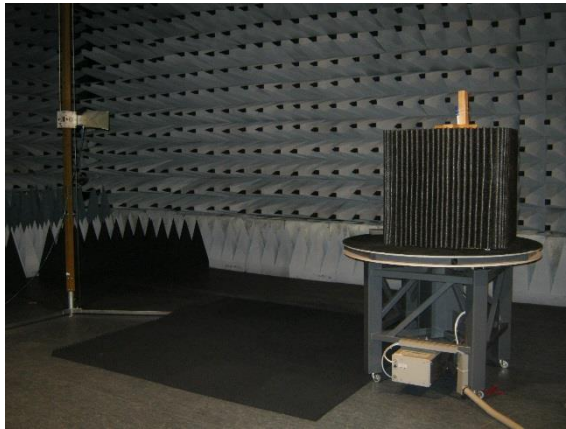
receiving/transmitting tested frequencies above 1 GHz (according to ANSI C63.10-2013)
