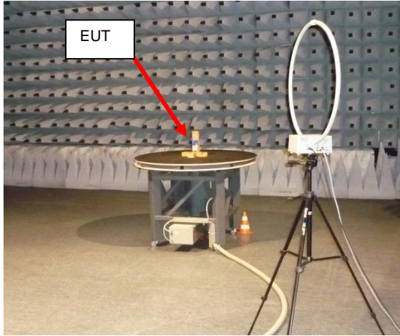
transmitting frequency range 9 kHz – 30 MHz
