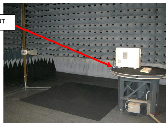
receiving/transmitting tested frequencies above 1 GHz (according to ANSI C63.10-2009)
