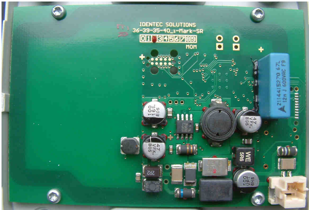
PCB view, side A (IMS-350-ER)
