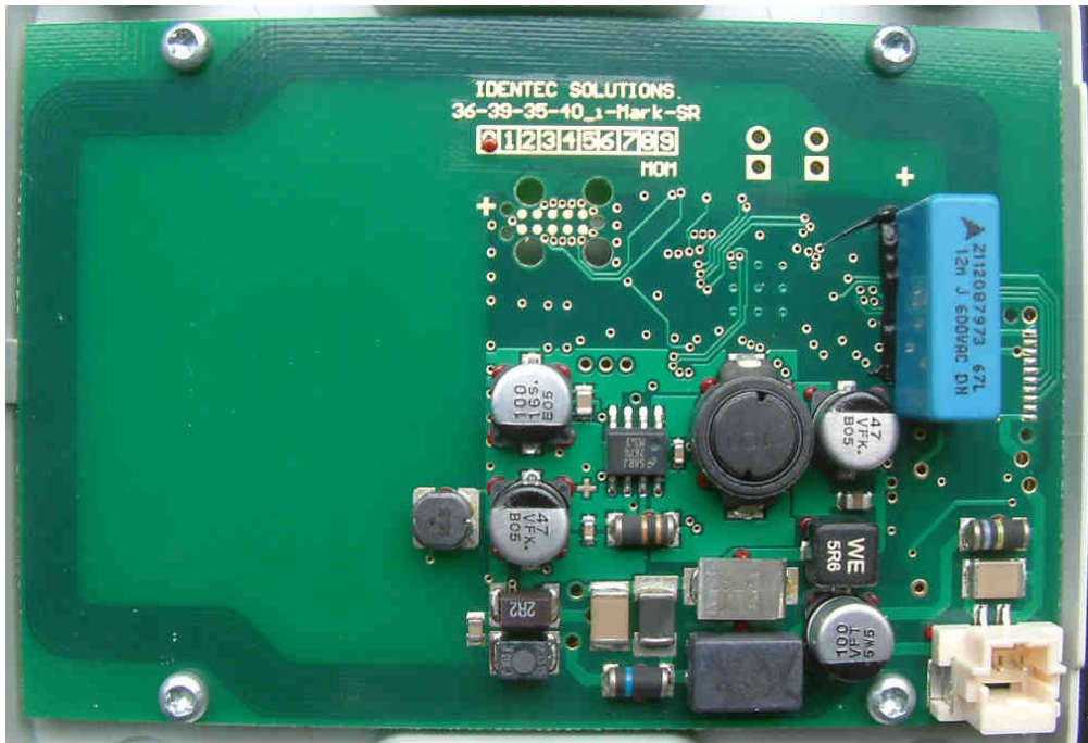
PCB view, side A (IMS-350)
