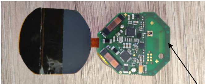
UHF antenna
