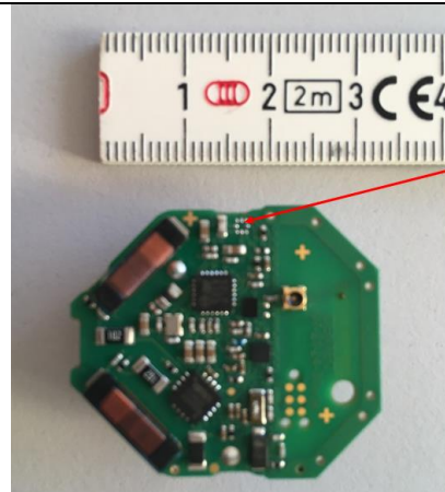
No-NFC version PCB
