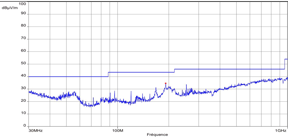
Vertical polarization
