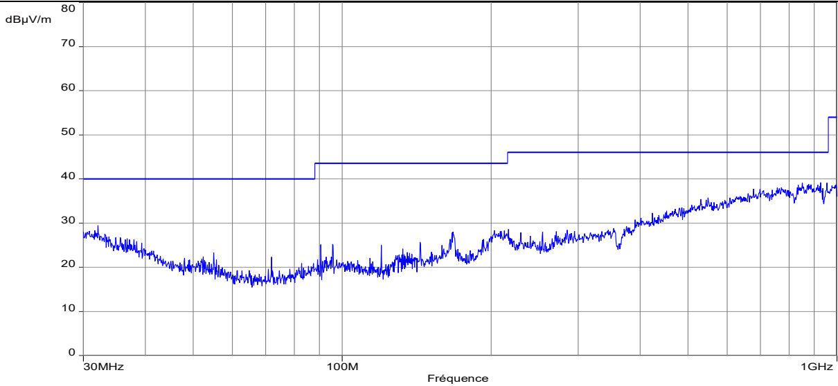
Vertical polarization
