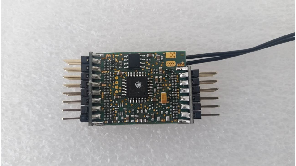
Figure 3: JETIREX10US – Top View
