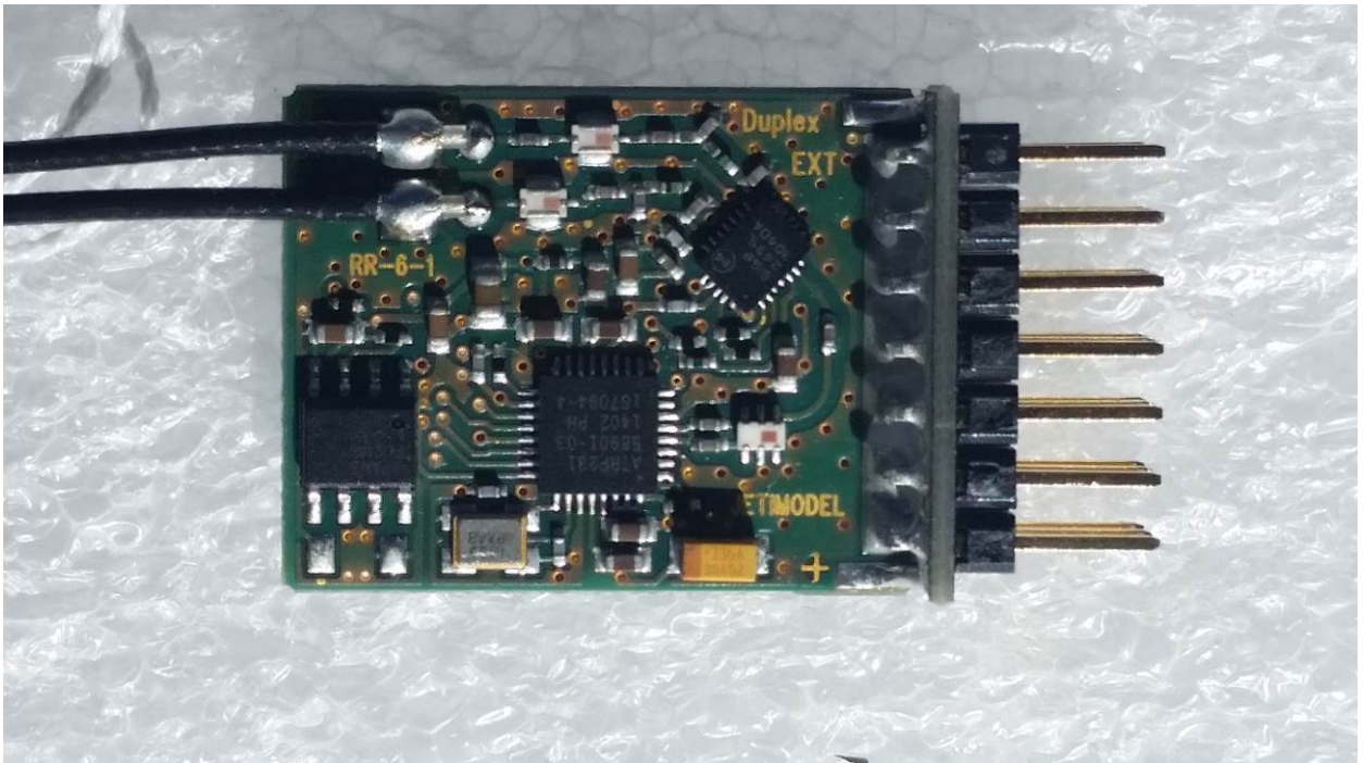
Figure 6: JETIREX7US – Bottom View
