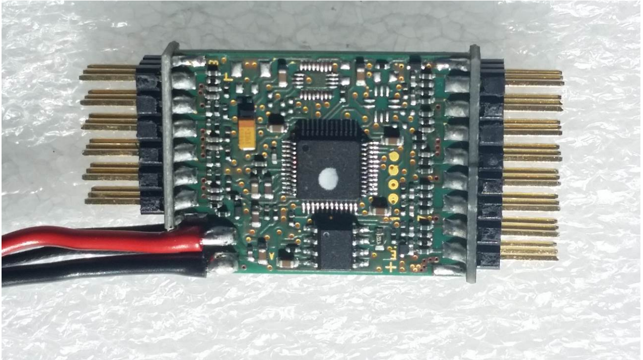
Figure 1: JETIREX12US – Top View
