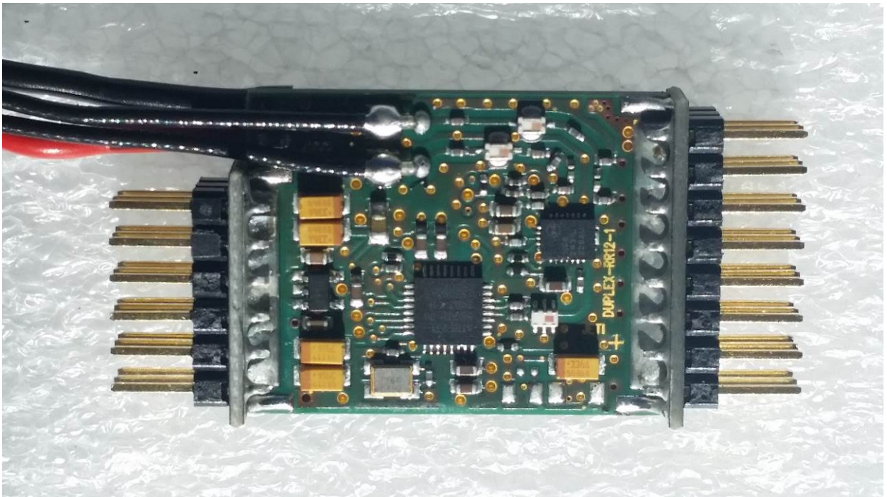
Figure 2: JETIREX12US – Bottom View
