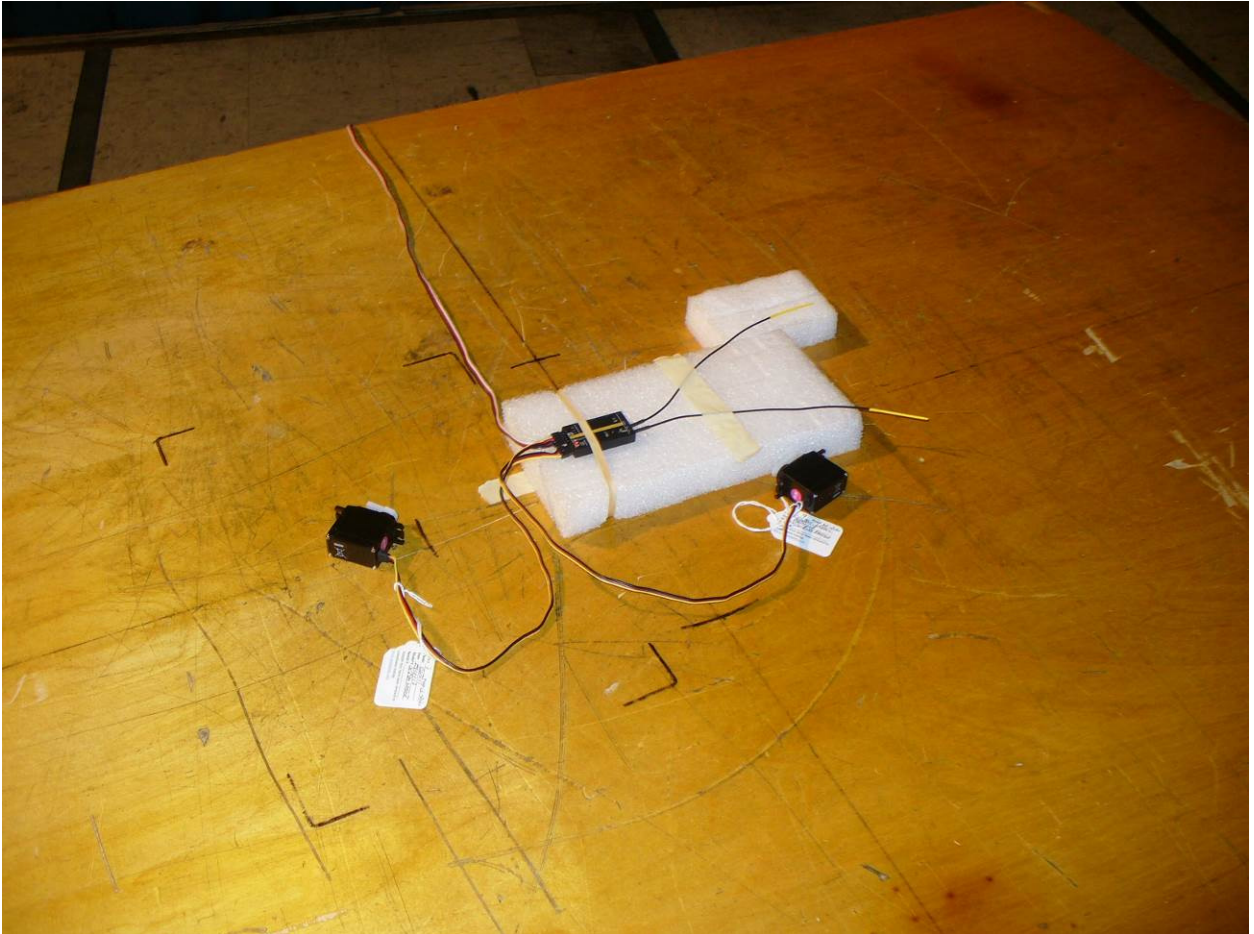
Figure 1: Radiated Emissions – Front View (Flat)
