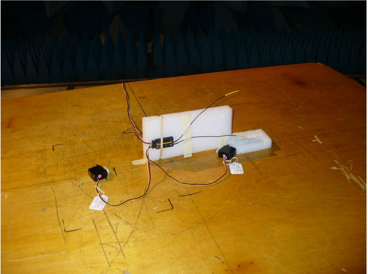
Figure 5: Radiated Emissions – Front View (Side)
