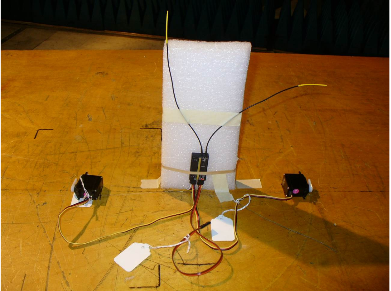
Figure 3: Radiated Emissions – Front View (Standing)
