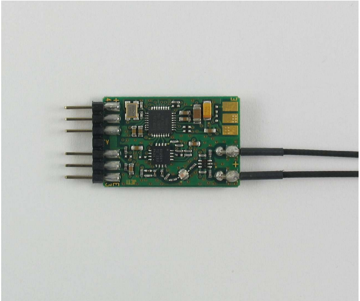
Figure 1: JETIR3US – PCB Top View
