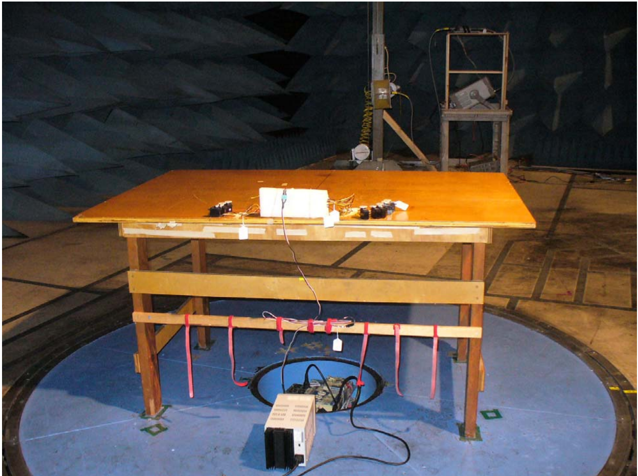
Figure 6: Radiated Emissions – Back View (EUT Side)
