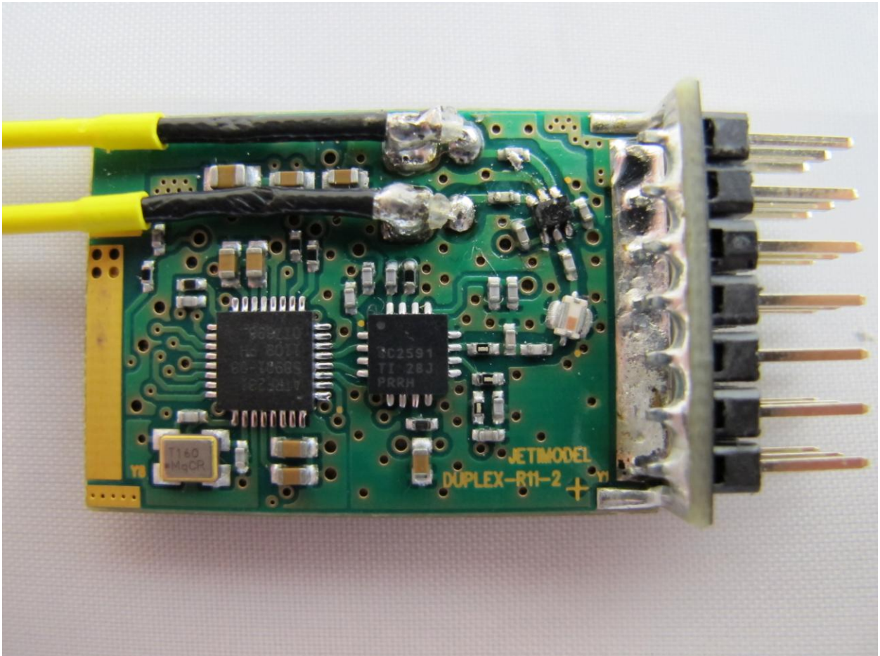
Figure 7: JETIR6iUS (PCB Top View)
