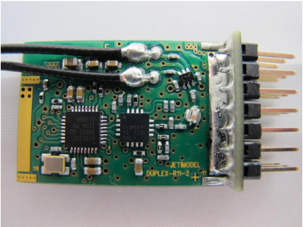
Figure 9: JETIR6LUS (PCB Top View)
