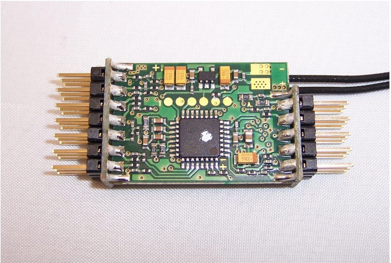
Figure 4: JETIR9US (PCB Bottom View)
