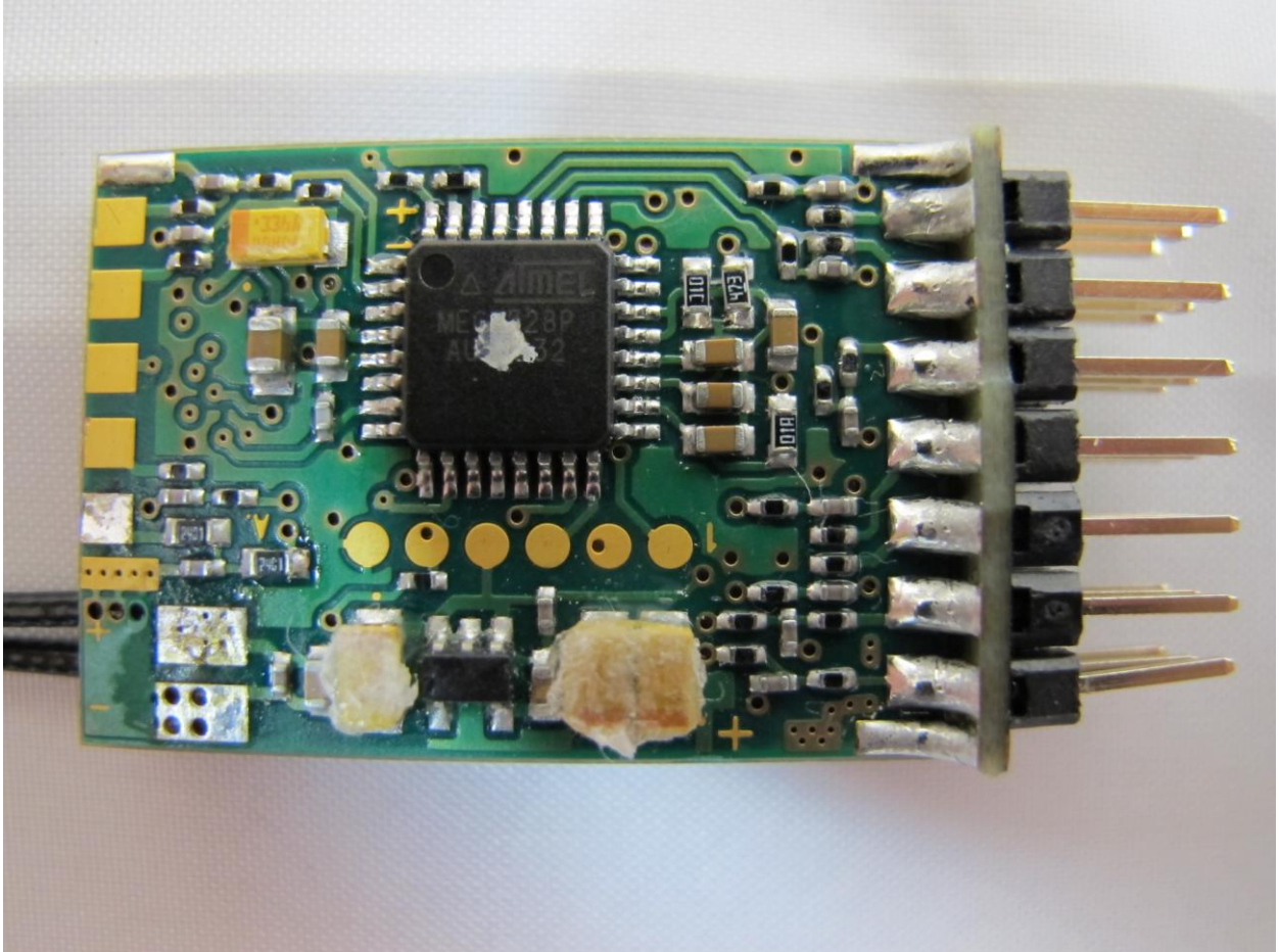
Figure 10: JETIR6LUS (PCB Bottom View)
