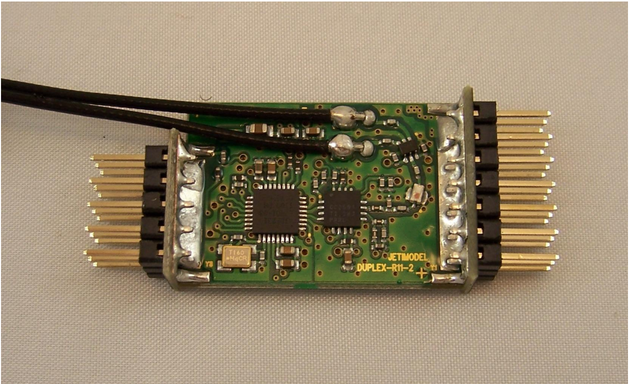
Figure 5: JETIR7US (PCB Top View)
