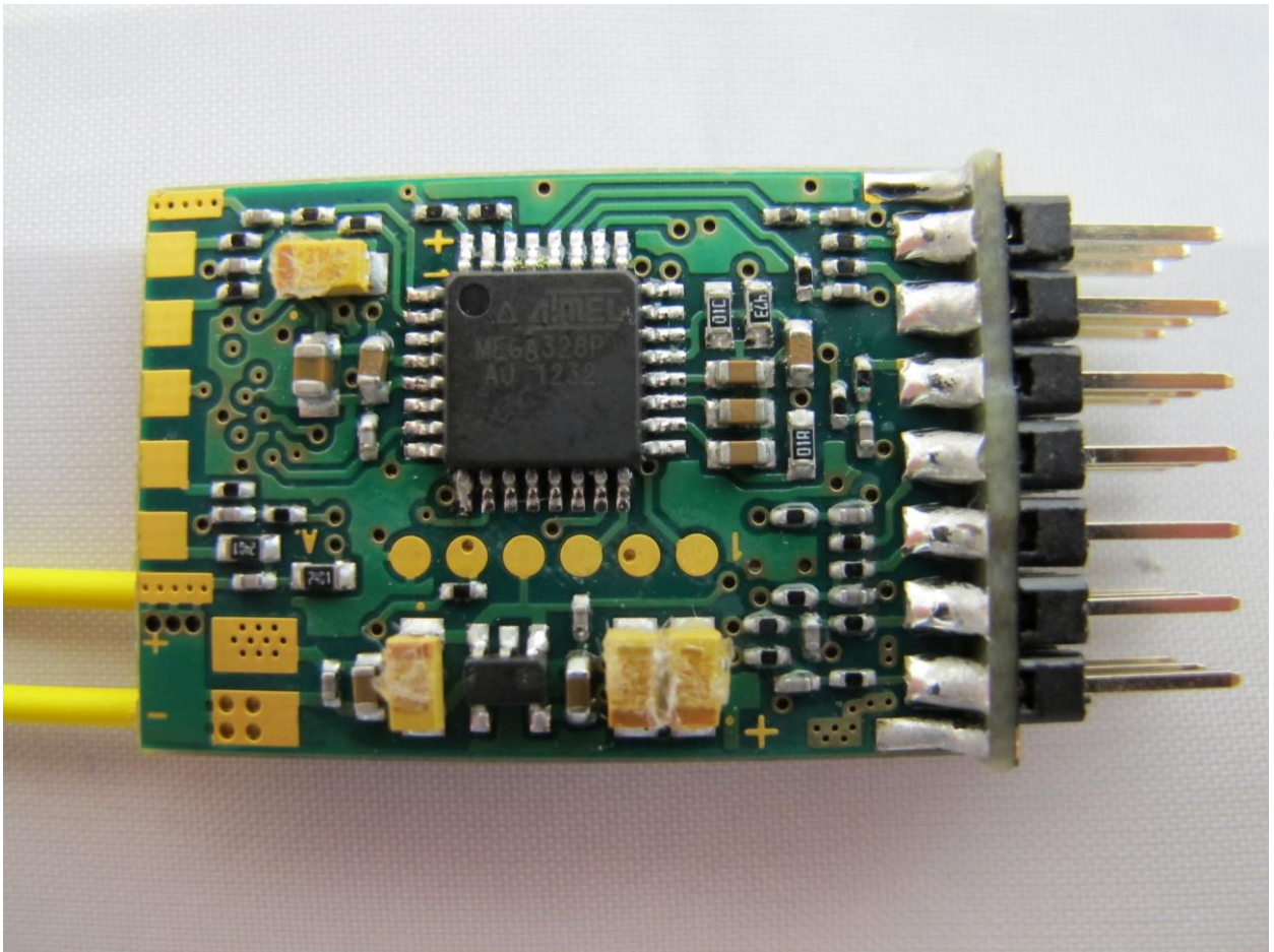
Figure 8: JETIR6iUS (PCB Bottom View)
