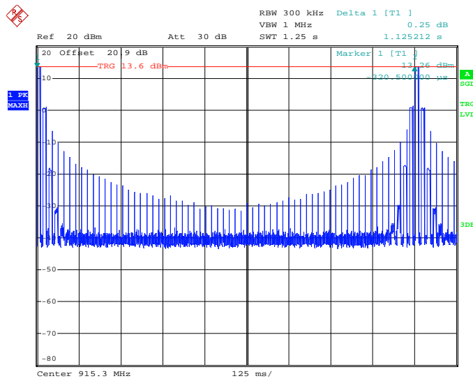
Figure 2.4.6-1: Channel Dwell Time Test Results
