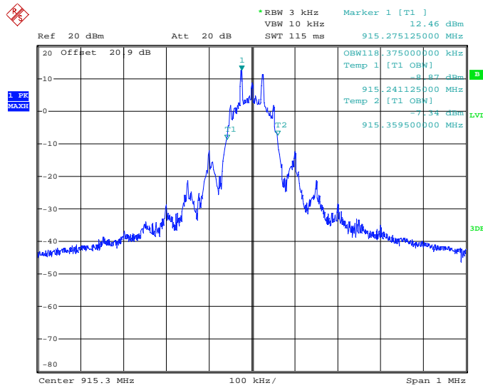
Figure 2.6.6- 1: 99% Bandwidth Test Results – Low Channel
