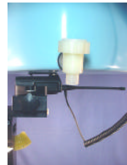
Body-worn SAR Test Setup with 1.0cm Belt-Clip
