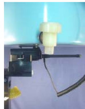
Body-worn SAR Test Setup with 1.0cm Belt-Clip
