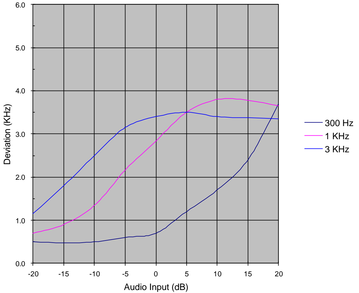
Modulation Limiting (25 KHz channel spacing : Negative Peak)
