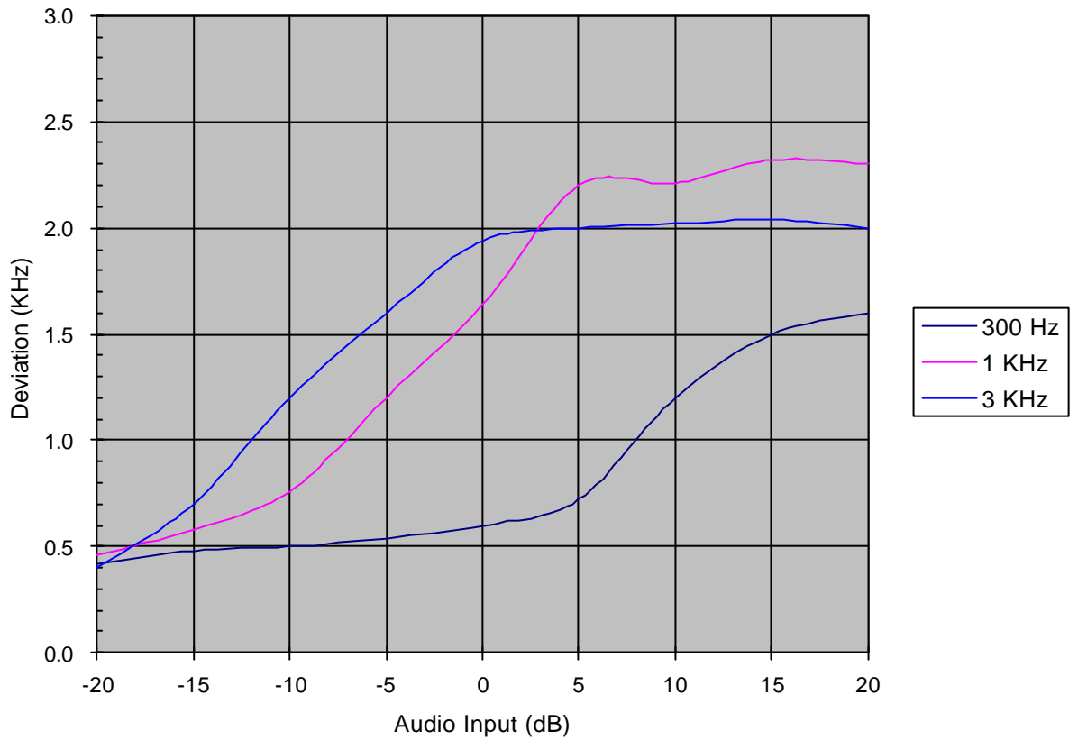
Modulation Limiting(12.5 KHz channel spacing : Positive Peak)
