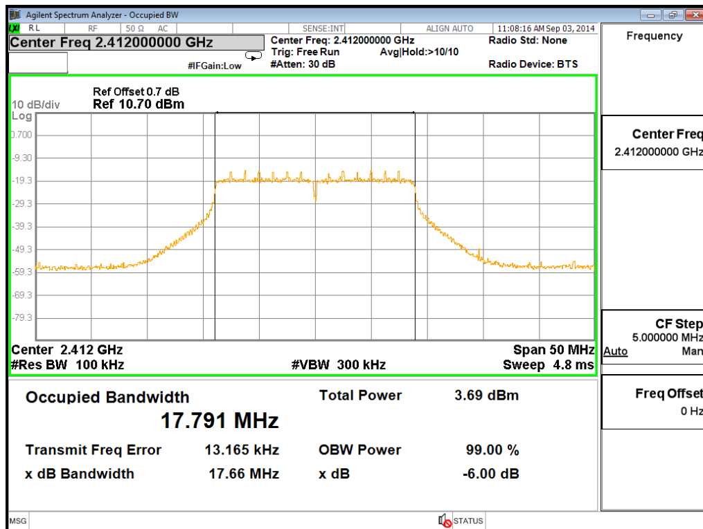
Channel 01 (2412MHz)
