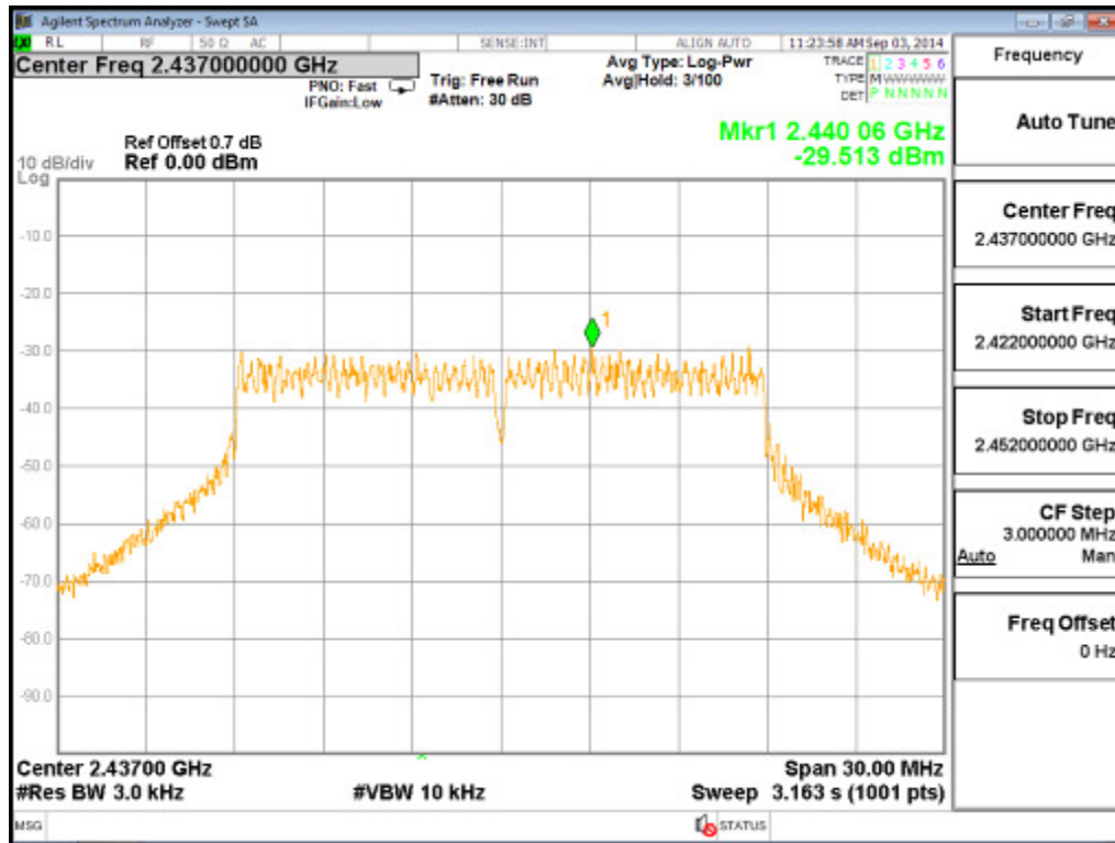
Channel 06 (2437MHz)
