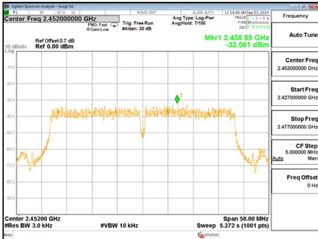
Channel 09 (2452MHz)
