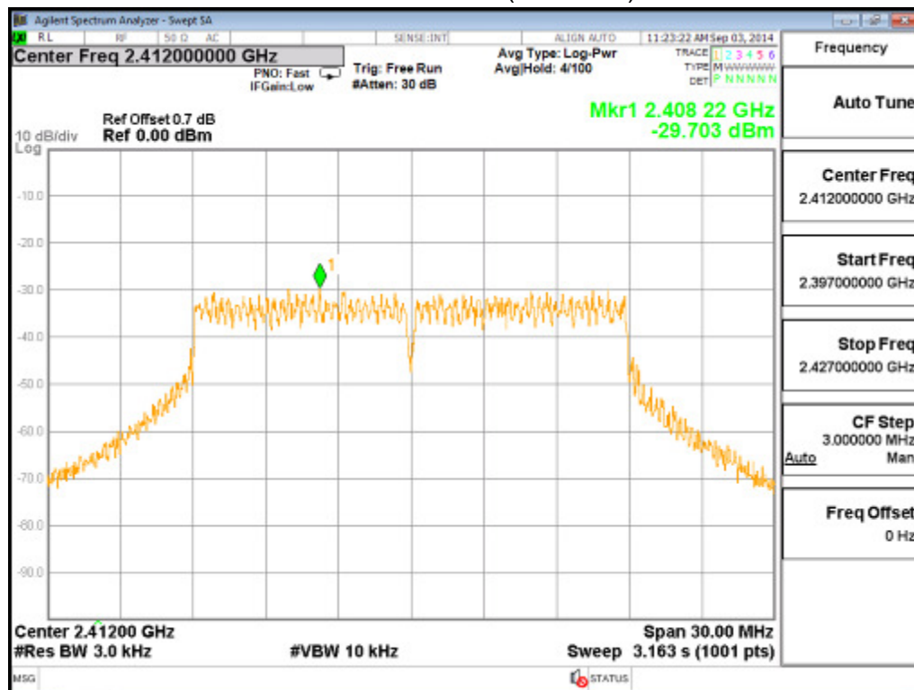
Channel 01 (2412MHz)
