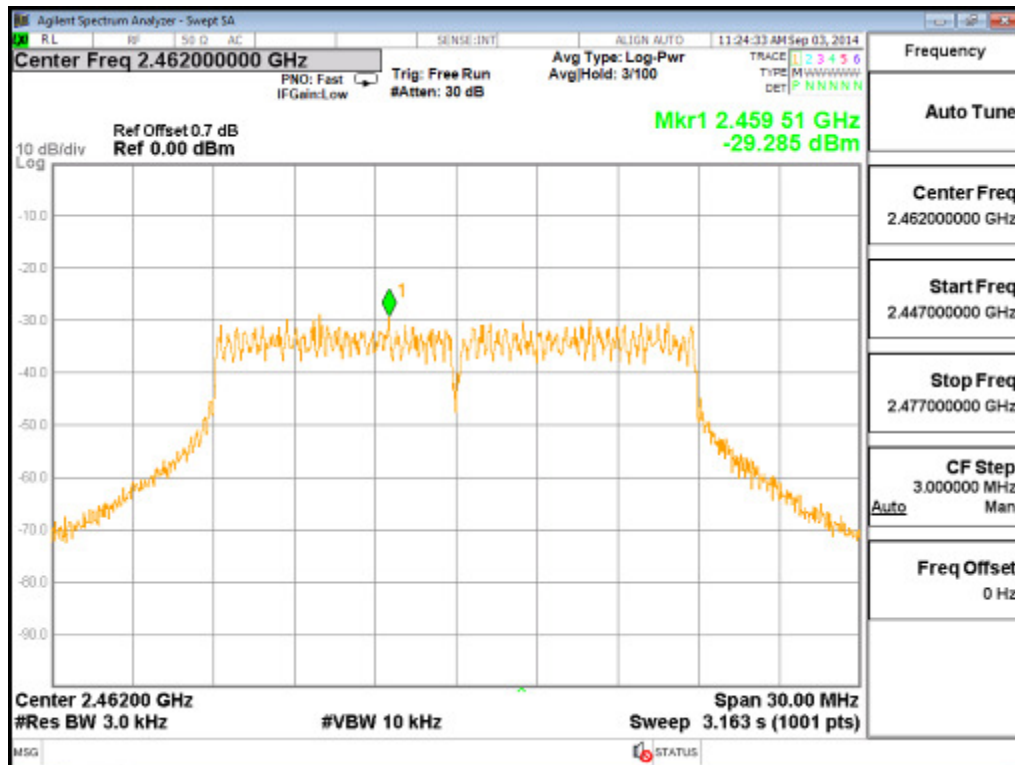
Channel 11 (2462MHz)
