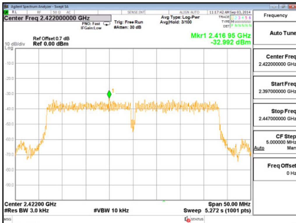
Channel 03 (2422MHz)
