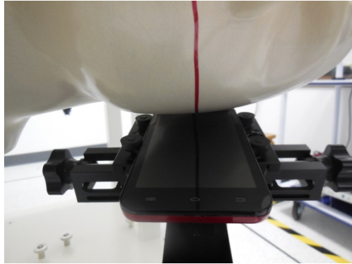
Band850, Band1900, WCDMA Band V, WIFI Test Setup Head Touch-Left Tilt-Left
