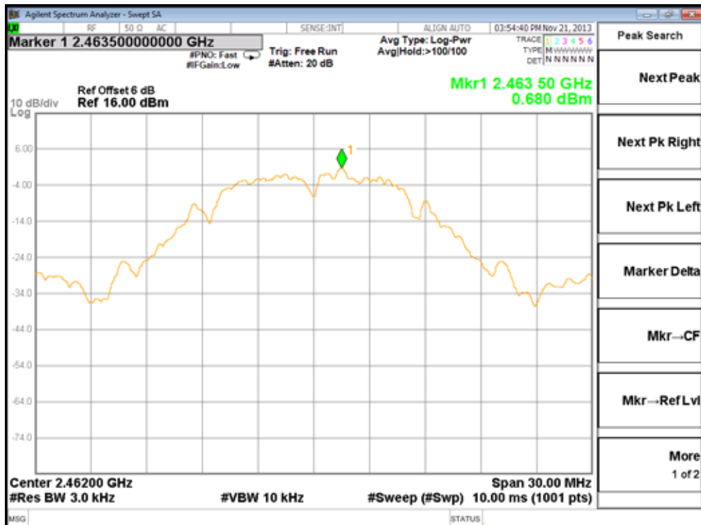
Channel 11 (2462MHz)
