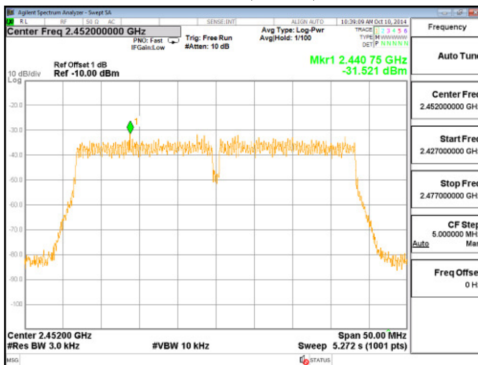
Channel 09 (2452MHz)
