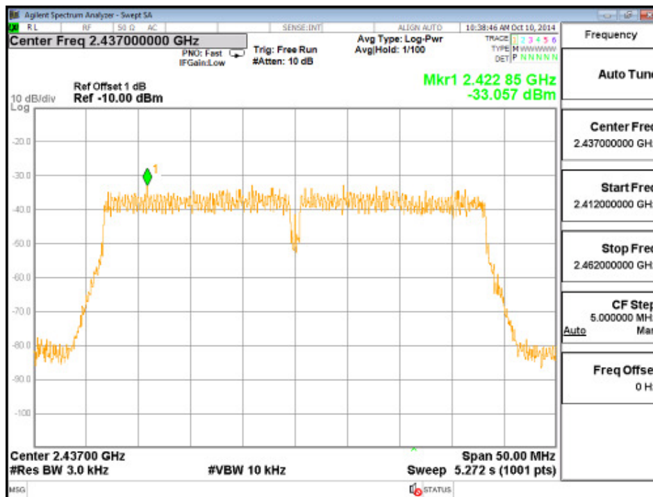
Channel 06 (2437MHz)
