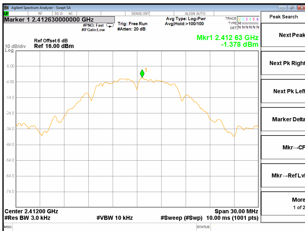
Channel 01 (2412MHz)
