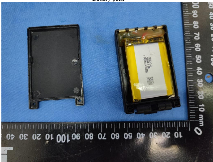
Battery pack
