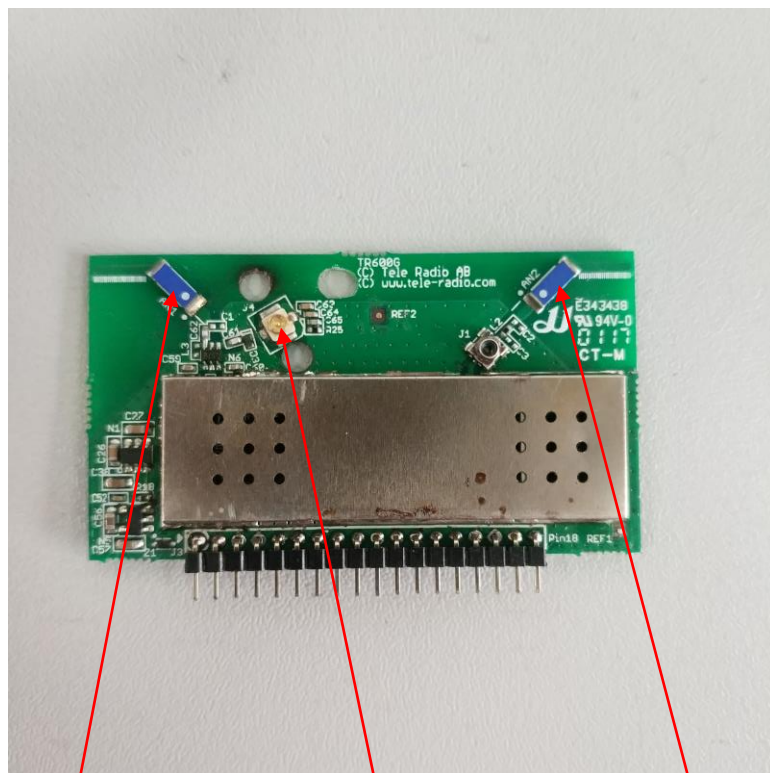
RF port of Antenna 2
