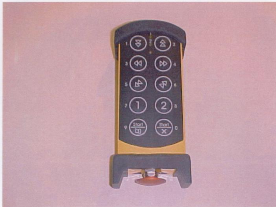
Photograph of EUT - Front view (Side view)
