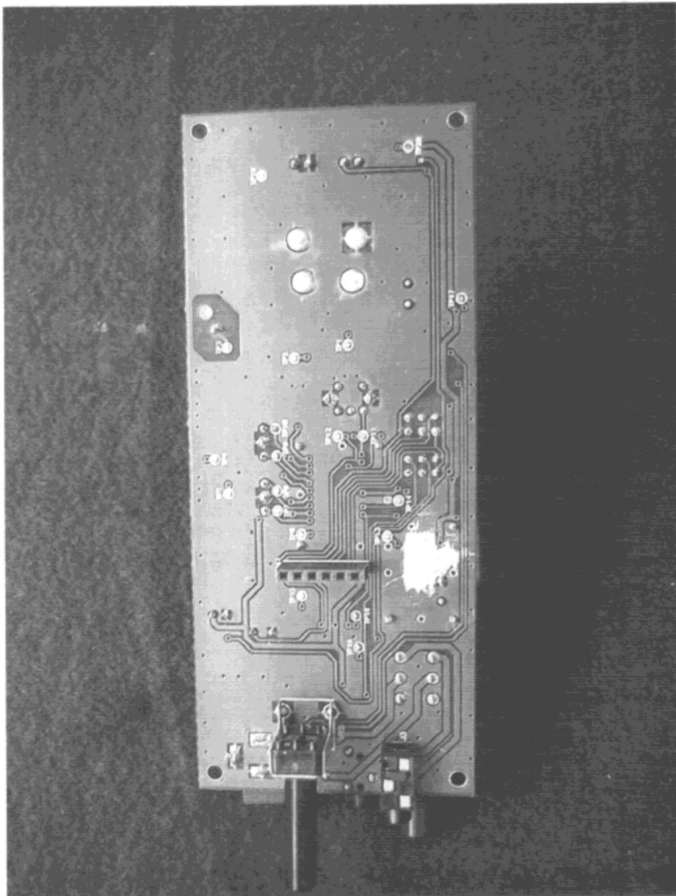
Image12-Base unit solder side-2
