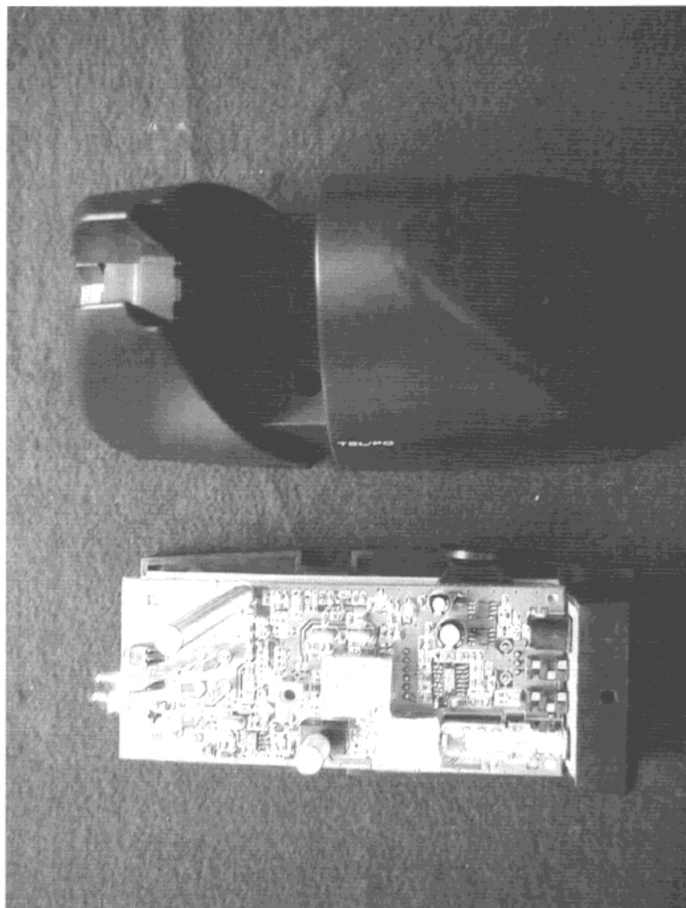
Image07-Base unit internal-1
