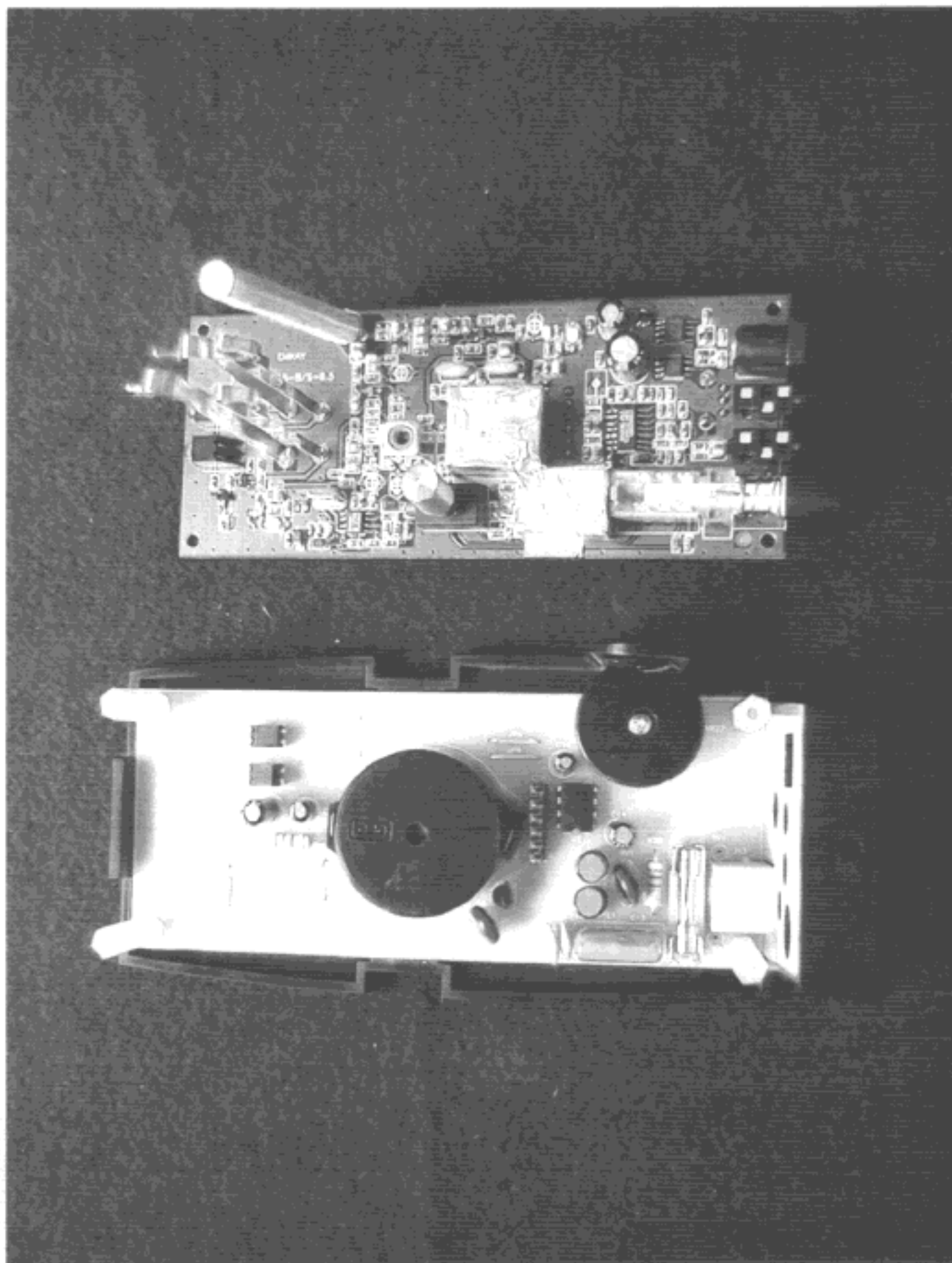
Image08-Base unit internal-2
