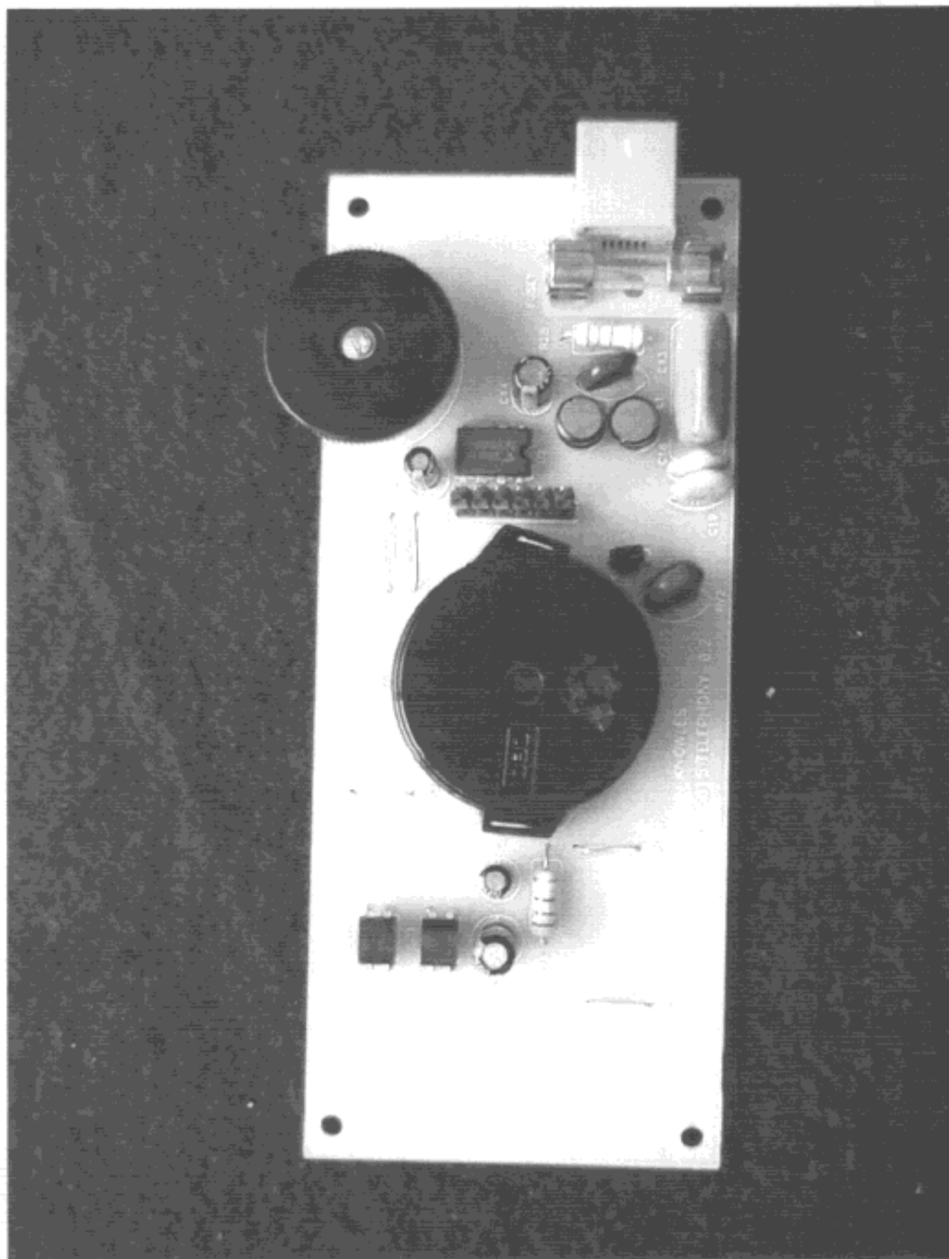
Image13-Base unit telecom terminal PCB component side
